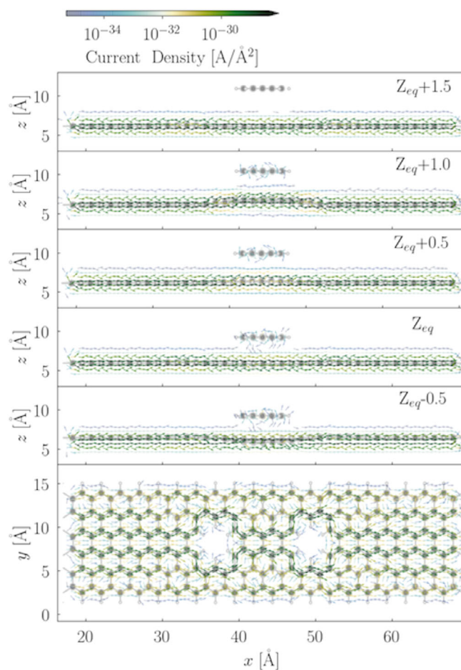
FIGURE 8 Quiver plot of the electronic current density projected on a real space grid. The local currents on the scattering region are reported for five systems, where the linker molecule is placed at the top position with different linker heights with respect to the defective zigzag graphene nanoribbons (ZGNRs). A 1 V bias voltage along the x-axis of the nanojunction plane is applied. For simplification, the current density is integrated along the y-axis of the nanojunction plane for the side view. The top view for the Z_{eq} conformation, integrated along the z-axis of the nanojunction plane, is shown in the bottom panel. The intensity of the current density is illustrated according to the color bar, where green indicates the high intensity and blue presents the low intensity
