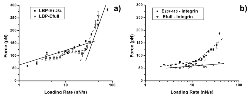
Figure 2. Single-molecule dynamic force spectroscopy data of full surface tick-borne encephalitis virus protein E and its fragments with laminin binding protein (LBP) (left) and human \alpha V\beta 3 integrin (right).
