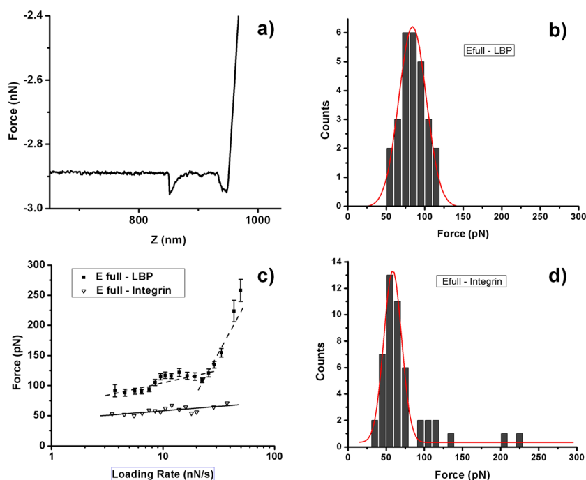
Figure 1. An example of force curve (a), single-molecule dynamic force spectroscopy data of full surface tick-borne encephalitis virus protein E–its putative cell receptors laminin binding protein (LBP) and human \alpha V \beta 3–integrin interactions (c) and specific bond rupture force distribution histograms obtained for the force loading rate in the range of 8–9 nN/s (b, d).
