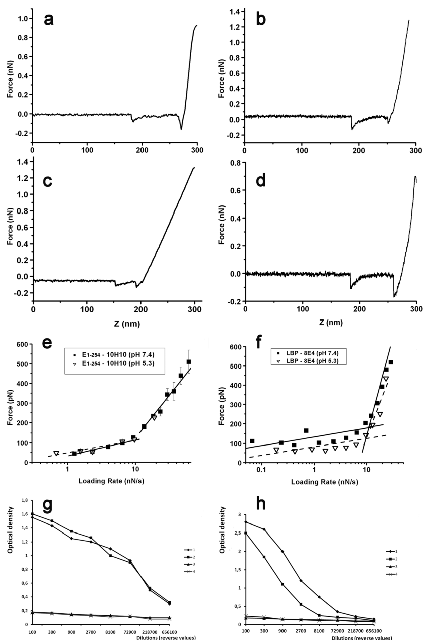
Figure 5. (a, b) Examples of force curves in the protein pairs E11–monoclonal antibodies (mAbs) 10H10 (a) and laminin binding protein (LBP)–mAbs 8E4 (b) at pH 7.4. (c, d) Examples of force curves for the same protein pairs as in (a) and (b), respectively, but at pH 5.3. (e, f) Single-molecule dynamic force spectroscopy data for interactions between antireceptor mAbs 10H10 and 8E4 and their complementary receptor regions in LBP and tick-borne encephalitis virus (TBEV) protein E molecules. (g, h) Corresponding immunoassay data. Left: 1—interaction of 10H10 mAb with recombinant protein E 1–254 of TBEV, pH 7.4; 2—interaction of 10H10 mAb with recombinant protein E 1–254 of TBEV, pH 5.3; 3—interaction of 10H10 mAb with Escherichia coli lysate transformed by empty PQE plasmid, pH 7.4 (negative control); 4—interaction of 10H10 mAb with E. coli lysate transformed by empty PQE plasmid, pH 5.3 (negative control). Right: 1—interaction of 8E4 mAb with recombinant protein LBP, pH 7.4; 2—interaction of 8E4 mAb with recombinant protein LBP, pH 5.3; 3—interaction of 8E4 mAb with E. coli lysate transformed by empty PQE plasmid, pH 7.4 (negative control); 4—interaction of 8E4 mAb with E. coli lysate transformed by empty PQE plasmid, pH 5.3 (negative control).
