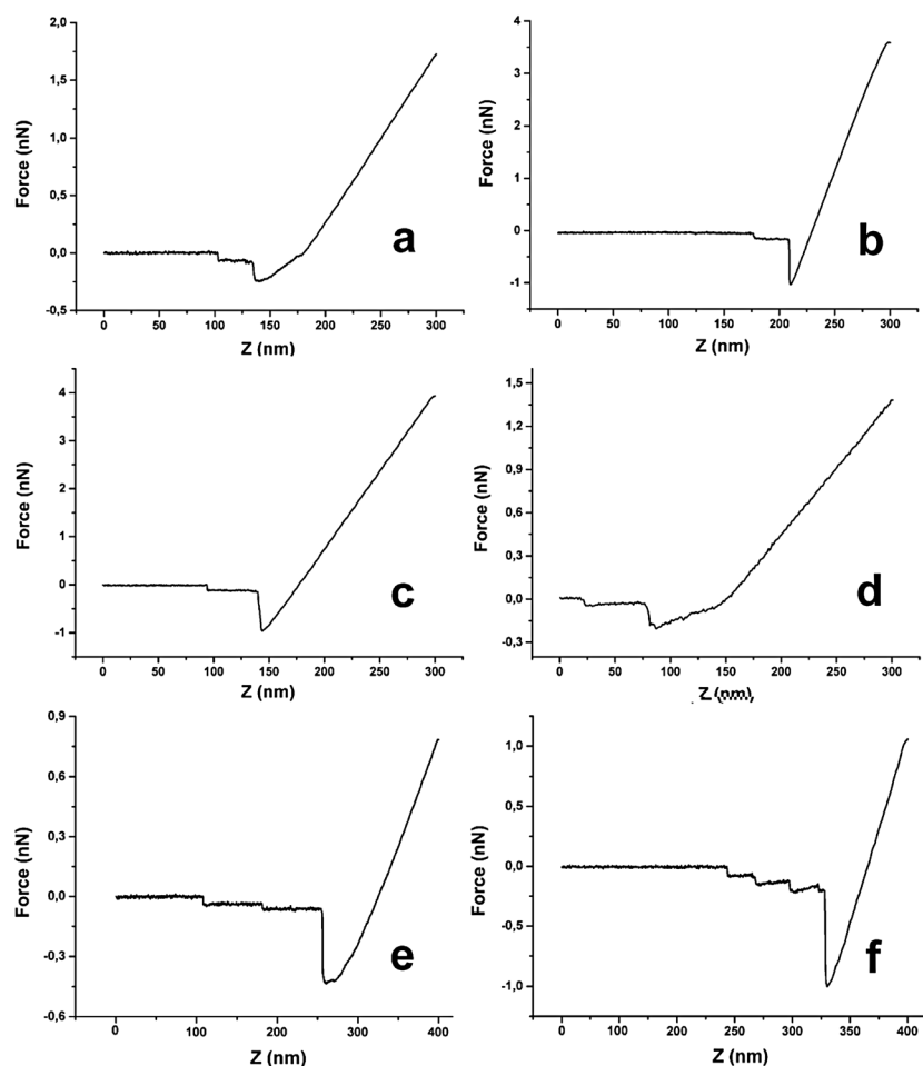
Figure 4. Examples of force curves exhibiting plateau(s) in the value of the force (“flat force curves”). (a) Laminin binding protein (LBP)-E 1-180 protein pair of West Nile virus (WNV) at pH 5.3, (b) LBP-E 53-126 protein pair of WNV at pH 5.3, (c) LBP deposited onto mica surface-atomic force microscopy (AFM) tip without any protein attached at pH 5.3, (d) LBP freely deposited onto freshly detached template-stripped gold surface (all other graphs present results obtained on mica surface)-AFM tip without any protein attached at pH 5.3 (curve recorded using Solver P47 Bio AFM, NT-MDT), (e) LBP-E 1-180 protein pair of tick-borne encephalitis virus at pH 5.3 (two force plateaus are seen), (f) LBP deposited onto mica surface-AFM tip without any protein attached at pH 7.4 (three force plateaus are seen).
