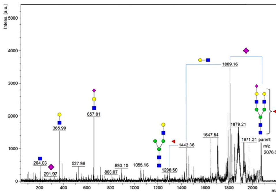
Figure 3. (C) MALDI TOF/TOF (LIFT) spectrum of representative ((Hex)2(HexNAc)2(Deoxy hexose)1(Neu5Ac)1 + (Man)3 (GlcNAc)2) N-glycan (with m/z 2076.6 in a negative ion mode) showing the typical fragmentation pattern of sialylated structure. The highest signal with m/z 1809.16 is referring to the loss of negatively charged sialic acid, leading to strong ionisation of residual structure in a positive ion mode. Another typical signal is the one with m/z 657.01, representing the N-acetyl-lactosamine residue terminated with sialic acid, which creates the typical mammalian N-glycan antennae. Glycan structures are shown according to CFG nomenclature.
