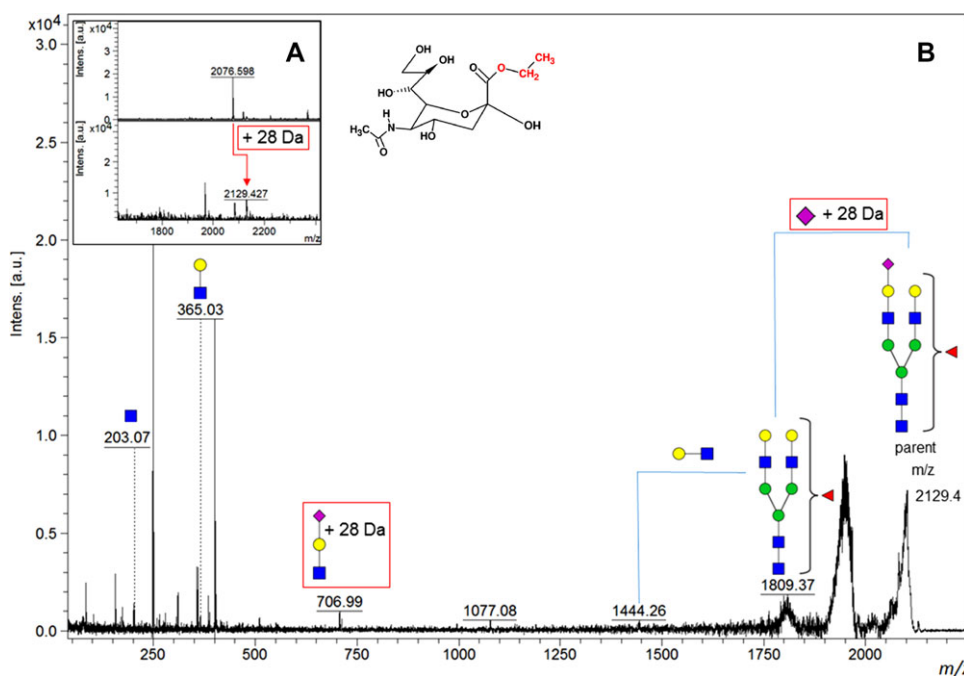
Figure 4. (A) Mass increment of 28 Da caused by ethyl esterification of a representative ((Hex)2(HexNAc)2(Deoxy hexose)1 (Neu5Ac)1 + (Man)3 (GlcNAc)2) N-glycan (with m/z 2076.6, [M - H]^- before the derivatisation and m/z 2129.4 [M + Na]^+ after). (B) MALDI TOF/TOF (LIFT) spectrum of the respective structure after the derivatisation. The loss of ethyl ester of sialic acid resulting in the signal at m/z 1809.4, as well as the presence of the signal at m/z 706.99 (N-acetyl-lactosamine with terminal ethyl ester of sialic acid) proved the selectivity of derivatisation and the presence of \alpha -(2,6)-linked sialic acid. The structure of ethyl esterified sialic acid is shown, as well. Glycan structures are shown according to CFG nomenclature.
