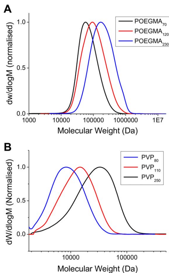
FIGURE 1 SEC analysis of RAFT-derived polymers. SEC was conducted in DMF and molecular weights calculated relative to PMMA standards. (A) POEGMA; (B) PVP. [Color figure can be viewed at wileyonlinelibrary.com ]
