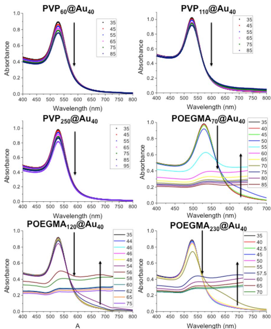
FIGURE 6 Assessment of the LCST behavior of polymer-coated gold nanoparticles. All measurements were conducted in PBS. Arrows indicate changes in spectral features and are intended to guide the eye only. [Color figure can be viewed at wileyonlinelibrary.com ]
