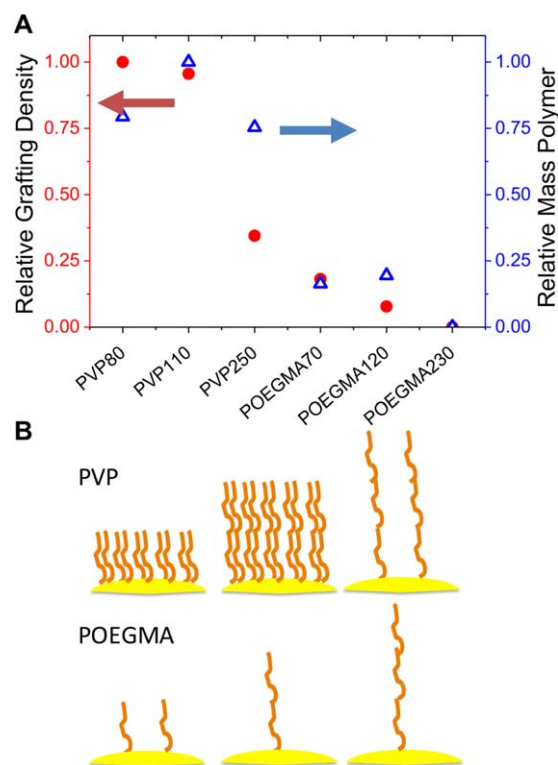
FIGURE 3 Grafting density comparison as estimated by XPS analysis. (A) Comparison of relative (assuming \text{PVP}_{80} = 1 ) grafting density (chains/unit area) and overall mass of polymer; (B) Schematic comparing relative grafting densities as a function of chain length and monomer type. [Color figure can be viewed at wileyonlinelibrary.com ]
