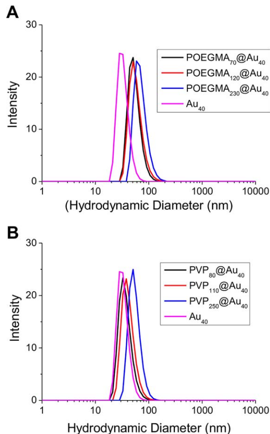
FIGURE 2 Dynamic light scattering analysis of polymer-coated gold nanoparticles. (A) POEGMA-coated nanoparticles; (B) PVP-coated nanoparticles. [Color figure can be viewed at wileyonlinelibrary.com ]
