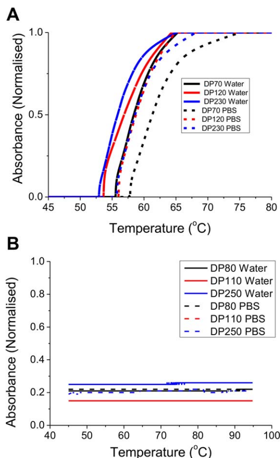
FIGURE 5 Turbidimetry analysis of polymers in Table 1. All measurements were conducted in water or PBS at 3 mg mL -1 . (A) POEGMA; (B) PVP. [Color figure can be viewed at wileyonlinelibrary.com ]
