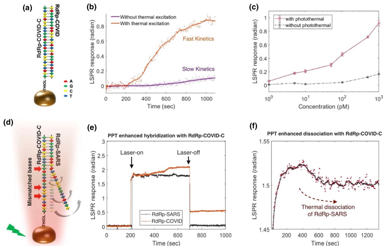
FIGURE 4 The surface-functionalised AuNl chips in the LSPR systems for specific viral sequence detection. 120 (a) Schematic illustration of the hybridisation of two complementary strands. (b) Realtime hybridisation of RdRp-COVID and its cDNA sequence (RdRp-COVID-C) with or without the thermoplasmonics enhancement. (c) PPT enhancement on RdRp-COVID sequence detection at different concentrations. The error bars refer to the standard deviations of LSPR responses after reaching the steady conditions following the buffer flushing. (d) Schematic illustration of inhibited hybridisation of two partially matched sequences. The red arrows indicated the mismatch bases of RdRp-SARS and functionalised cDNA of RdRp-COVID. (e) Discrimination of two similar sequences with PPT heat. The laser was applied at 200 s and switched off at 700 s. (f) RdRp-SARS sequence dissociation from the immobilised RdRp-COVID-C sequence. The original phase responses (red dots) and the corresponding smoothed means (black curve) are shown
