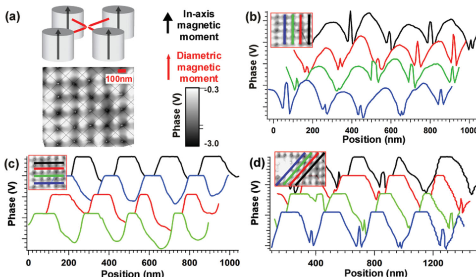
Figure 7. (a) MFM map of about 1\mu\text{m} \times 1\mu\text{m} area of the sample with nanoholes filled with \text{Fe}_3\text{O}_4 nanoparticles. The corresponding magnetic moments of interest are depicted in the inset (top: red arrow for the diametric magnetic moment, black arrow for the in-axis magnetic moment). (b–d) Profiles extracted from the MFM image (a): (b) vertically across the nanoholes, (c) horizontally across the white lobes and (d) diagonally across the nanoholes. The locations are depicted in the respective insets (color coded black, red, green, blue).
