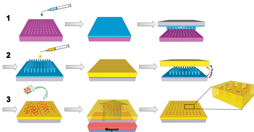
Figure 1. Schematic showing the steps involved in (1) fabricating PUS nanopillar structures from a silicon mold (2) printing of PAN nanoholes patterns from the PUS mold (3) filling of \text{Fe}_3\text{O}_4 nanoparticles into the nanoholes: a solution of \text{Fe}_3\text{O}_4 nanoparticles was drop-casted onto the hole arrays; the particles were dragged into the holes by a magnet. Stray particles remaining on the surface were washed away with excess solvent.
