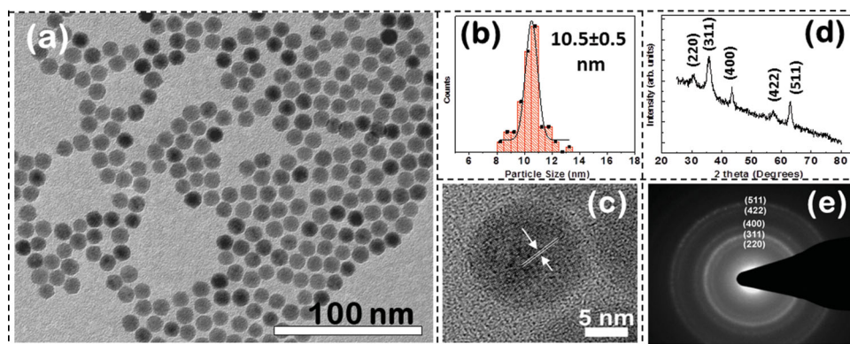
Figure 2. Bright-field TEM image of as-synthesized \text{Fe}_3\text{O}_4 nanoparticles (a), the corresponding particle size distribution (b), HRTEM image of a single \text{Fe}_3\text{O}_4 nanoparticle (c), XRD pattern (d) and SAED image of the \text{Fe}_3\text{O}_4 nanoparticles (e).
