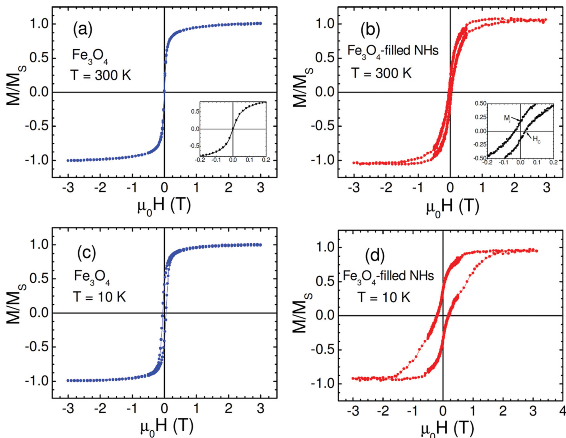
Figure 6. Magnetic hysteresis (M-H) loops taken at 300 K and 10 K for the as-synthesized Fe 3 O 4 nanoparticles (a, c) and for the Fe 3 O 4 -filled nanohole film (b, d). The insets of Figure 6a and b show the enlarged low-field M-H curves.
