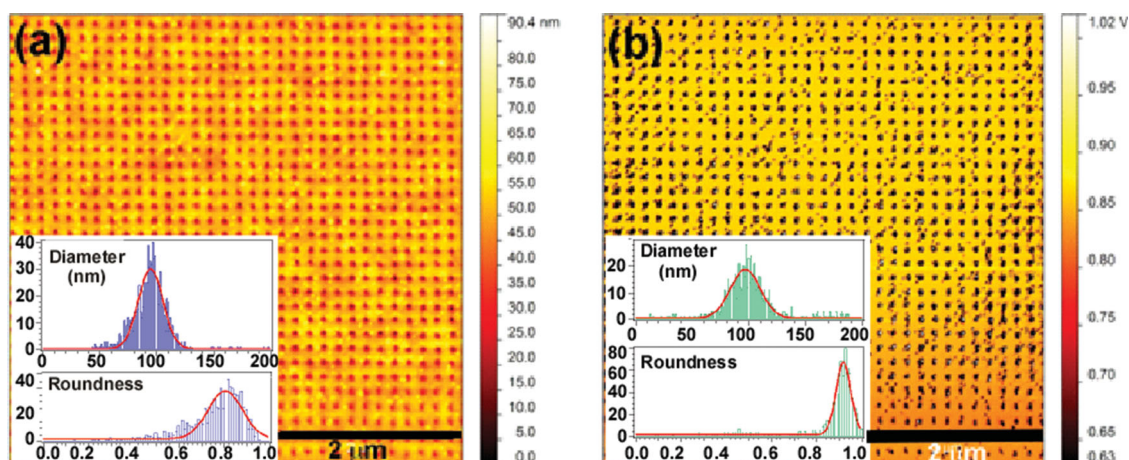
Figure 4. (a) AFM topography image of a nano-patterned array of holes filled with 10 nm \text{Fe}_3\text{O}_4 nanoparticles; (b) MFM image of the same region. The size distribution of the nanoholes as extracted from AFM topography image of a nano-patterned array of holes (top inset in a) and MFM image of the nano-patterned array of holes filled with 10 nm \text{Fe}_3\text{O}_4 nanoparticles (top inset in b). Roundness distribution of the nanoholes signals as extracted from AFM topography image of a nano-patterned array of holes (bottom inset in a) and MFM image of the nano-patterned array of holes filled with 10 nm \text{Fe}_3\text{O}_4 nanoparticles (bottom inset in b).
