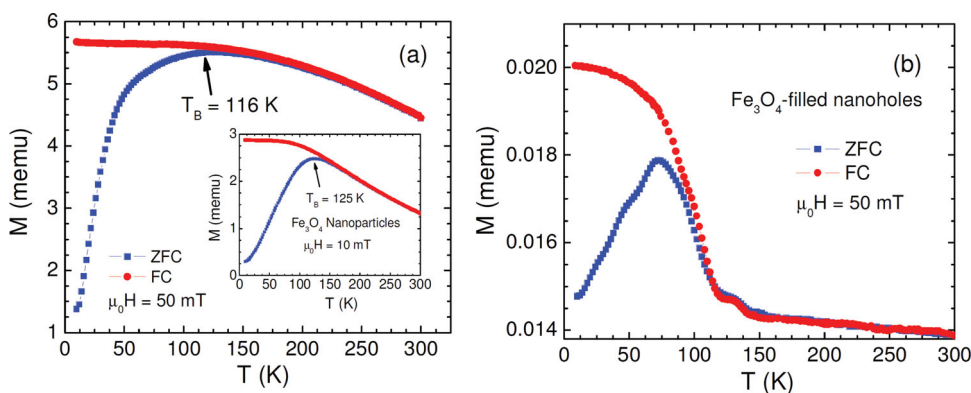
Figure 5. Temperature dependence of ZFC and FC magnetization (M–T) taken at a field of 50 mT for the \text{Fe}_3\text{O}_4 nanoparticles (a) and for the \text{Fe}_3\text{O}_4 -filled nanohole film (b). The inset of Figure 5a shows the M–T dependence for an external magnetic field of 10 mT for the \text{Fe}_3\text{O}_4 nanoparticles.
