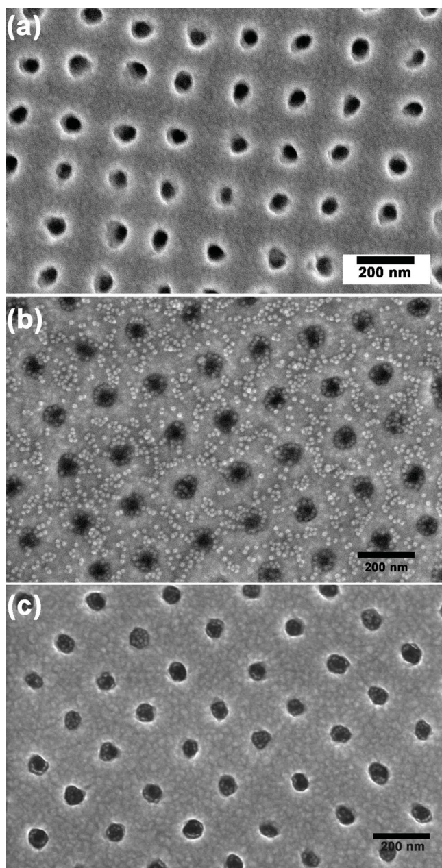
Figure 3. SEM images show arrays of nanoholes (a) before and (b) after filled with \text{Fe}_3\text{O}_4 nanoparticles and (c) after removing stray particles.
