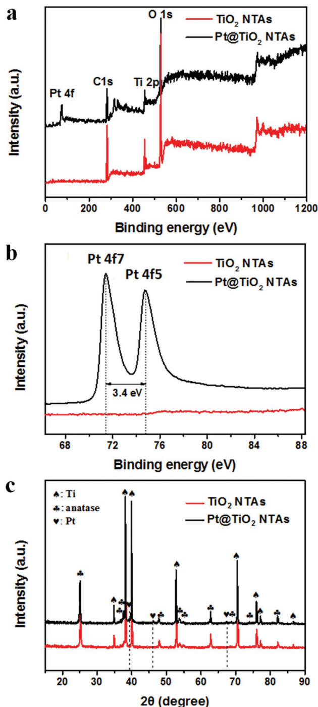
Figure 3. a) XPS spectrum and b) high resolution XPS spectra of pristine \text{TiO}_2 and EPD-reduced Pt@ \text{TiO}_2 NTAs using 0.4 \times 10^{-3} M chloroplatinic acid solution. c) XRD patterns of pure \text{TiO}_2 NTAs and EPD-reduced Pt@ \text{TiO}_2 NTAs using 0.4 \times 10^{-3} M chloroplatinic acid solution.
