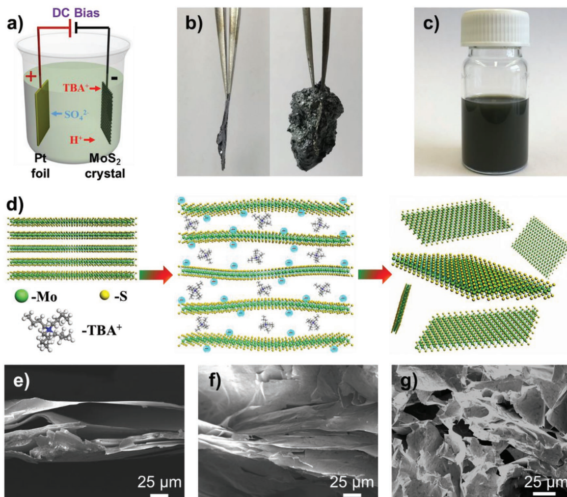
Figure 1. Electrochemical exfoliation of MoS 2 flakes: a) schematic illustration of an electrochemical exfoliation cell, b) photographs of bulk MoS 2 crystal (left) and expanded MoS 2 crystal after exfoliation (right), c) MoS 2 flakes dispersed in propylene carbonate, d) schematic illustration for mechanism of electrochemical exfoliation, and e–g) SEM images of MoS 2 crystal at the edges after applying a bias of −5 V for 0, 1, and 10 min in organic TBA·HSO 4 electrolyte, respectively.
