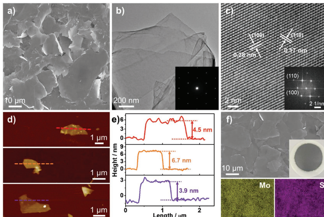
Figure 2. Morphological characterizations of exfoliated MoS 2 flakes and thin film. a) SEM image of exfoliated MoS 2 flakes on Si/SiO 2 wafer, b,c) HRTEM images and corresponding diffraction patterns (inset) of a few-layered MoS 2 flake, d) AFM images, e) height profiles of exfoliated MoS 2 flakes taken from the supernatant, and f) top-view SEM image of MoS 2 thin film and corresponding EDS elemental mapping analysis. Inset: Photograph of MoS 2 thin film on a PTFE membrane (50 mm in diameter).
