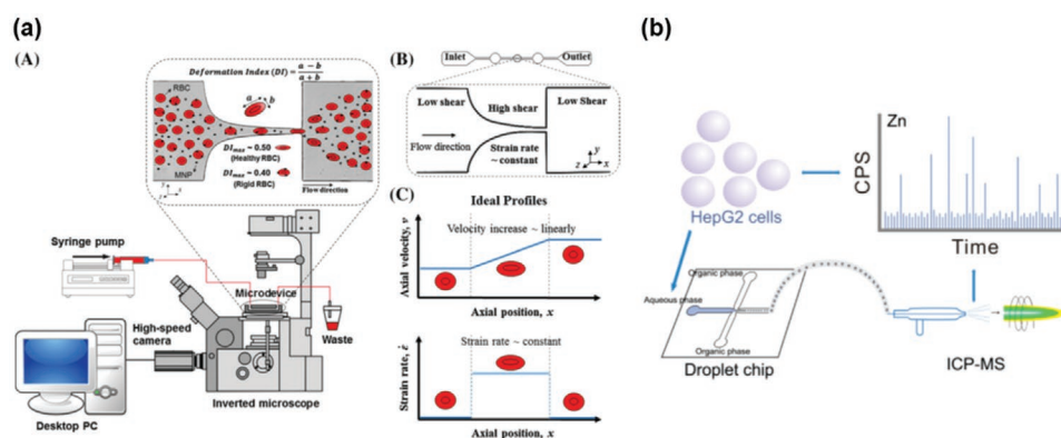
Figure 4. Microfluidic devices for single cell analysis: a) Hemocompatibility of red blood cells in contact with MNPs through deformation index assessment, A) schematic view of microfluidic setup, B) Microchannel device geometry with the zoom of the hyperbolic channel, C) graphical representation of the fluid-induced condition profiles that occur in the hyperbolic channel. Reproduced with permission. [90] Copyright 2016, Springer Nature. b) Microfluidic drop chip combined with ICPMS system for determination of zinc in single cell. Reproduced with permission. [94] Copyright 2017, ACS Publications.
