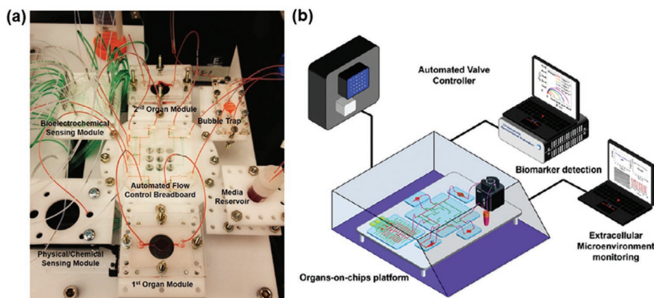
Figure 8. Multisensor-integrated organ-on-a-chip platforms for automated and continuous in situ monitoring of organoids. a) Photograph of the integrated platform including microbioreactors, breadboard, reservoir, bubble trap, physical sensor and electrochemical biosensors; b) Schematic of the full system organ-on-a-chip platform encased in an in-house designed benchtop incubator. Reproduced with permission. [132] Copyright 2017, PNAS.
