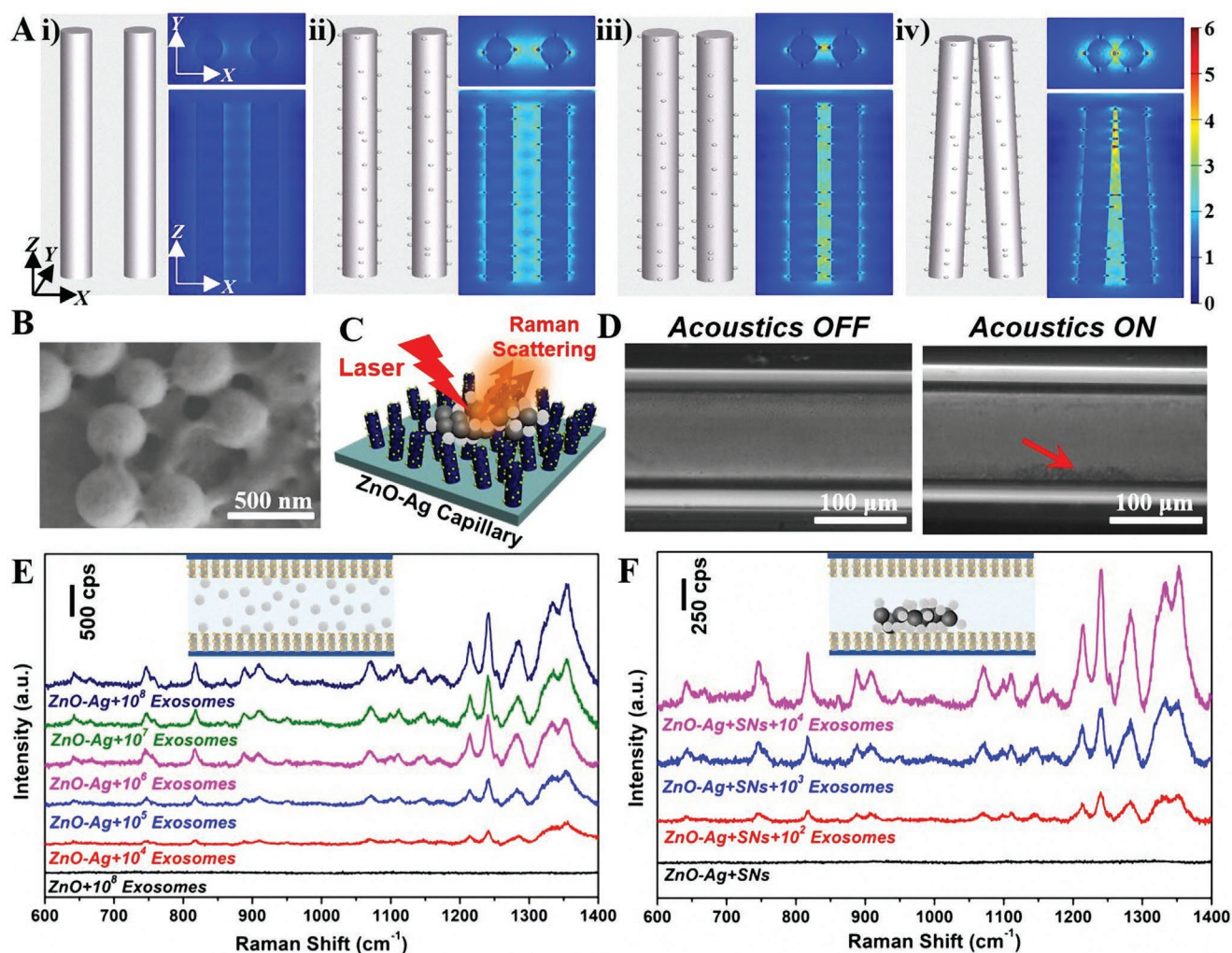
Figure 6. Acoustofluidics-assisted SERS detection of exosomes. A) FDTD simulations showing the electromagnetic field distributions of different nanoarray structures. i) pristine nanorods with a gap distance of 200 nm with limited electromagnetic field enhancement; ii) ZnO–Ag nanorods with a gap distance of 200 nm showing strong electromagnetic field enhancement; iii) ZnO–Ag nanorods with a gap distance of 100 nm showing further magnified electromagnetic field enhancement; iv) Tilted plasmonic nanorods with ends clustered together showing dramatically enhanced electromagnetic field. B) SEM images of SNs-400 after interaction with exosomes under mild sonication treatment. C) Schematic diagram showing the nanoparticle-assisted SERS sensing mechanism of the ZnO–Ag capillary toward exosomes. D) Top view microscope image of solution with exosomes which are bound to silica nanoparticles (SNs-400) when the SAW was OFF and ON (10 V, 7.65 MHz). E) SERS spectra of exosomes with concentrations ranging from \approx 10^4 to 10^8 \mu\text{L}^{-1} using ZnO–Ag capillary without the assistance of silica particles (10 V, 7.65 MHz). F) SERS spectra of exosomes with concentrations ranging from \approx 10^2 to 10^4 \mu\text{L}^{-1} using the nanoparticle-assisted acoustofluidic method (10 V, 7.65 MHz).
