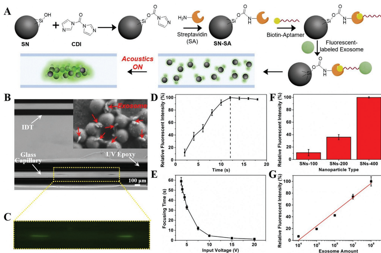
Figure 4. Acoustofluidics-assisted immunofluorescent detection of exosomes. A) Schematic diagram showing the immunoassay process. B) Top view microscope image of solution with exosome-conjugated SNs-400 when the SAW was ON. The inset is a SEM image showing the interactions of exosomes with SNs-400. C) Enlarged image of solution when excited by a 365 nm laser. D) Relative fluorescent intensity changes of exosome-conjugated SNs-400 as enrichment time increased when using an input voltage of 7.5 V. The dashed line indicates the focusing time when the fluorescent intensity reached the maximum level. E) Focusing time changes of exosomes-conjugated SNs-400 as the input voltage increased. F) Comparison of different-sized nanoparticles for immunofluorescent detection of exosomes. G) Relative fluorescent intensity of exosomes-conjugated SNs-400 at different concentrations of exosomes and the fitted linear relationship between exosome quantity and fluorescent intensity ( y = 24.12x - 96.2 , R^2 = 0.973 ). The concentrations of exosomes and silica particles in (B–F) were 10^6 exosomes \mu\text{L}^{-1} and 0.2 \mu\text{g} \mu\text{L}^{-1} , respectively. The driving voltage and frequency are 10 V and 7.5 MHz, respectively, in these tests unless otherwise stated.
