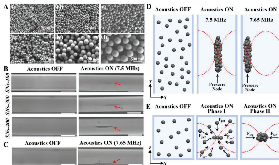
Figure 3. Demonstration of the acoustofluidic enrichment of different-sized silica nanoparticles inside the glass capillary. A) SEM images of SNs-100, SNs-200, and SNs-400 with particle sizes around 100 nm (i, ii), 200 nm (iii, iv), and 400 nm (v, vi), respectively. B) Top view of particle solution inside the glass capillary when the acoustics is OFF and ON at 7.5 MHz. Scale bar = 100 \mu m. C) Top view of solution with SNs-400 when the acoustics is OFF (left) and ON by changing the applied frequency from 7.5 to 7.65 MHz (right). Scale bar = 100 \mu m. D) Schematic illustration showing the use of acoustics for directed transport of silica nanoparticles. E) Typical acoustic particle trapping configuration when interdigital transducers emit sound in a direction perpendicular to the flow. F_{prf} and F_{sec} indicate the primary radiation forces and the secondary forces, respectively.
