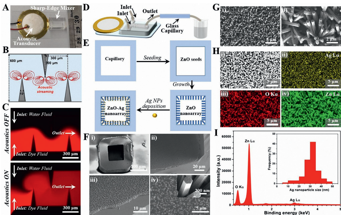
Figure 5. Acoustofluidic synthesis of functional plasmonic nanoarray inside square-shaped glass capillaries. A) A photograph of an acoustofluidic sharp-edge mixer device with a ruler for scale. B) The design parameters and the proposed acoustic streaming pattern of the sharp-edge micromixer. C) Fluorescent images for comparing the mixing performance of water fluid and dye fluid (Rhodamine B) when the acoustic transducer is OFF (top) and ON (bottom). D) Schematic diagram showing the operation of the acoustofluidic sharp-edge mixer for plasmonic nanoarray synthesis. E) Schematic workflow showing the synthesis process of the plasmonic nanoarray inside the glass capillary. F) SEM images showing the structures of the ZnO nanoarray. The inset in (F-iv) indicates the smooth surface of the ZnO nanorods. G) SEM images showing the structures of the ZnO–Ag nanoarray. H) SEM image (i) and the corresponding element mapping profiles of Ag (ii), O (iii), and Zn (iv). I) EDS spectrum of ZnO–Ag nanoarray, and the inset is the size distributions of Ag from 200 random particles under TEM.
