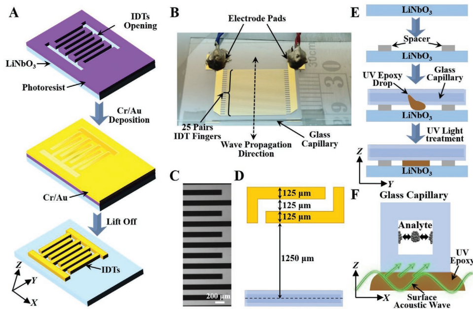
Figure 2. Development of the SAW-based acoustofluidic enrichment platform. A) Schematic of the fabrication process showing the formation of IDTs on a piezoelectric LiNbO 3 substrate for surface acoustic wave generation. Objects are not drawn to scale. B) A photograph of the SAW-based acoustofluidic device used in the experiments with a ruler for scale. C) Structural pattern of IDTs under optical microscope. D) Design parameters of SAW-based acoustofluidic enrichment setup. E) Schematic diagram showing the integration process of the glass capillary onto the LiNbO 3 substrate. F) Schematic of surface acoustic wave propagation for sample enrichment inside the glass capillary.
