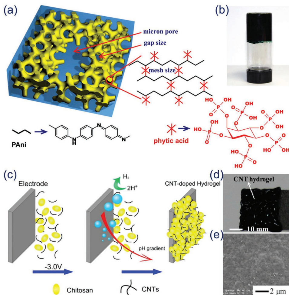
Figure 2. a) Schematic representation of 3D microporous PANI hydrogel network. b) PANI hydrogel inside a glass. Reproduced with permission. [104] Copyright 2012, Proceedings of National Academy of Sciences. c) Fabrication of self-assembled CNT-hydrogel onto a carbon paper electrode through the simultaneous electrodeposition of both CNT and chitosan. d) CNT hydrogel fabricated on carbon paper; and e) SEM image of CNT hydrogel-modified paper. Reproduced with permission. [109] Copyright 2012, American Chemical Society.
