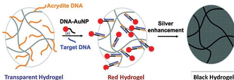
Figure 8. The use of DNA-functionalized hydrogels and AuNPs for colorimetric DNA detection. When the target DNA is present, the color of the transparent gels changes to red. Signal amplification can be accomplished by lowering \text{Ag}^+ in the presence of AuNPs to coat the gel with metallic silver. Reproduced with permission. [129] Copyright 2010, American Chemical Society.
