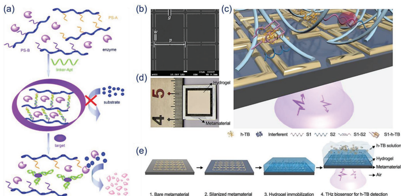
Figure 7. a) Aptamer–target binding resulting gel disassembly. Reproduced with permission. [211] Copyright 2010, Wiley-VCH. b) SEM image of the bare THz metamaterial. c) Schematic representation of h-TB sensing by the THz biosensor. d) The physical image of the THz biosensor. e) Experimental procedure of the proposed strategy. Reproduced with permission. [223] Copyright 2021, American Chemical Society.
