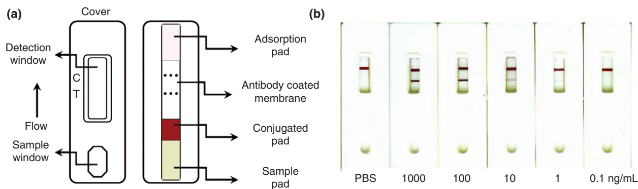
FIGURE 5 | A lateral flow assay using colloidal gold for colorimetric, visual detection is depicted in (a, C: Control, T: Test). The assay demonstrated a qualitative increase in signal in the Test region with increasing target concentration (b). (Reprinted with permission from Ref 56. Copyright 2010 Elsevier)
