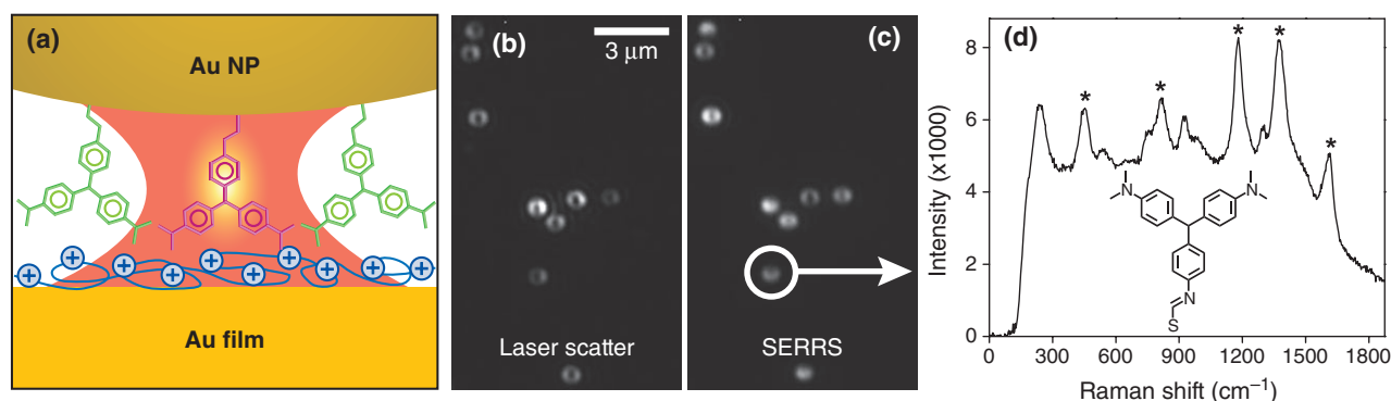
FIGURE 9 | Gold nanoparticles (NPs) in close proximity to gold film create localized regions of field enhancement that can be used for stimulated surface enhanced resonance Raman scattering (SERRS, a). The NP-film SERRS hot spots are generated with 100% yield, as is indicated by the fact that each NP in the laser scatter image (b) also appears in the SERRS image (c). A SERRS spectrum with characteristic peaks from a Raman reporter molecule can be collected from each film-coupled NP (d). (Reprinted with permission from Ref 104. Copyright 2010 ACS)
