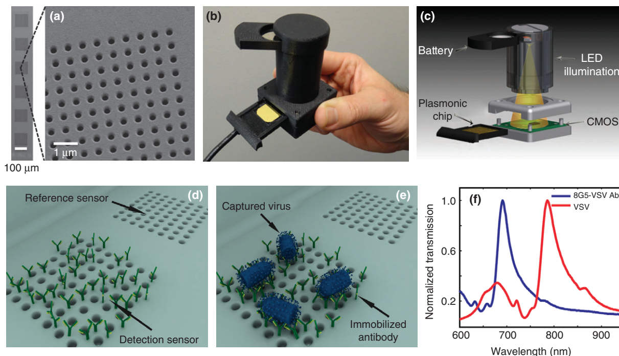
FIGURE 6 | Plasmonic nanopores (a) exhibit extraordinary optical transmission (EOT) when illuminated collinearly due to excited plasmonic modes defined by the grating order of the nanopore array. A handheld miniature nanopore array sensing device is shown in (b and c). An example of nanopore sensing is shown in (d–f) where the presence of a virus (red plot) is detected by a shift in the wavelength of the EOT from a nanopore sensing array containing antibodies targeting the virus (blue plot). (a–c) (Reprinted with permission from Ref 65. Copyright 2014 NPG) (d–f) (Reprinted with permission from Ref 68. Copyright 2010 ACS)
