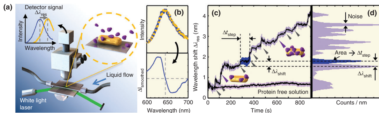
FIGURE 3 | Single nanoparticles (NPs) can be spectroscopically characterized using a dark field microscope (a). The localized surface plasmon resonance (LSPR) of a NP shifts when protein attaches to the surface of the NP (b). This LSPR shift was tracked over time to reveal step-wise attachment of single proteins to the NP being analyzed (c, d). (Reprinted with permission from Ref 29. Copyright 2012 ACS)
