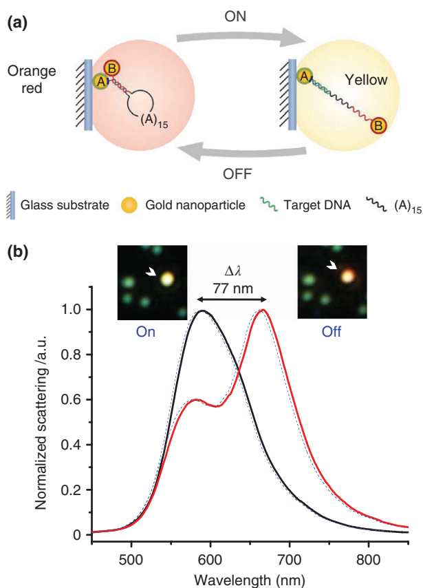
FIGURE 7 | A plasmonically coupled nanoparticle (NP) dimer designed to detect DNA is depicted in (a). When target DNA is present the separation distance between the NPs increases and produces a blue shift in the coupled localized surface plasmon resonance of the NP dimer (b). The NP dimer in the inset dark field images (b) is indicated by an arrow. (Reprinted with permission from Ref 77. Copyright 2013 Wiley)
