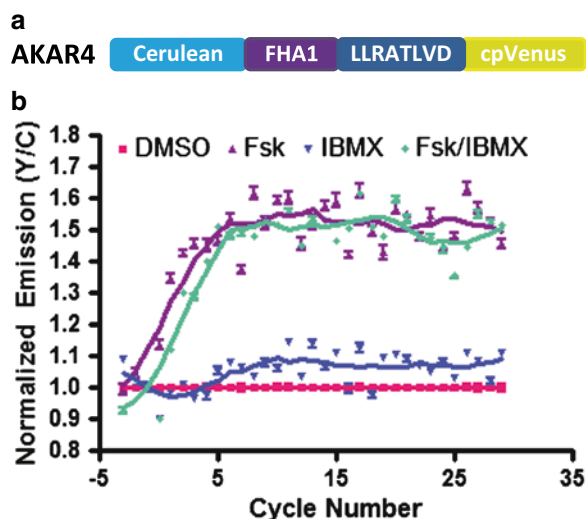
Fig. 2 High throughput activity assay based on an improved AKAR (AKAR4) (a). Design of AKAR4 (b). Representative time-course curves depicting changes in emission ratios (Y/C) of HEK293T cells expressing AKAR4, treated with DMSO (1 %), Forskolin (50 \mu M), IBMX (100 \mu M), and a combination of Forskolin and IBMX (50 \mu M, 100 \mu M respectively). 1 cycle = 16 s. Error bars represent standard deviation ( n=4 )
