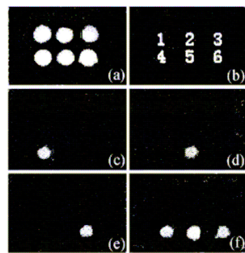
Fig. 1. Image of a fiber-optic biosensor array obtained by a CCD camera. (a) Image with white light transmitted through the untreated end of the array; (b) background fluorescence image at 685 nm taken with 633 nm excitation, no fluorescence signal observed. The numbers show the order of the fibers in the array; (c)—(e) fluorescent image of the fiber-optic biosensor array acquired after hybridization with p53 target (c), N-ras target (d), Rb1 target (e); (f) a mixture of p53 , N-ras , and Rb1 targets.
