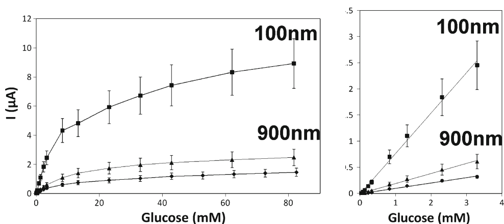
Fig. 5 Calibration curves for glucose at Pt electrodes functionalized with poly(pyrrole-NTA) and successively incubated with \text{CuCl}_2 ( 10 \text{ mM} ) and histidine-tagged GOx: (diamonds) in the absence of nanobeads, (triangles) with 900-nm-diameter beads, and (squares) with 100-nm nanobeads; (right) plot of the linear part. (Measurements performed by chronoamperometry at E=0.6 \text{ V} vs SCE, 0.1 \text{ M PBS} , \text{pH } 7 , 25^\circ\text{C} )
