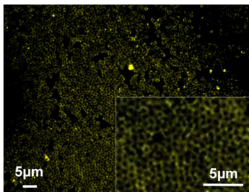
Fig. 3 Fluorescence microscope images of an electrode modified with a biotinylated tyrosinase followed by incubation with FITC-labeled avidin. The electrode was previously functionalized with poly(pyrrole-NTA)/Cu 2+ electrogenerated on 900-nm beads that were dissolved after the polymer formation. The control experiment was performed with nontagged enzymes and exhibited negligible fluorescence
