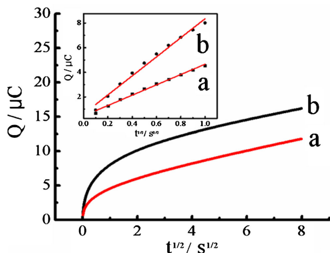
Fig. 6 Q-t curves of the bare GCE (a) and the AuNPs/CuS-Gr/GCE (b) in 0.1 mM K_3[Fe(CN)_6] containing 1.0 M KCl. The inset shows Q-t^{1/2} curves for the GCE (a) and the AuNPs/CuS-Gr/GCE (b)
