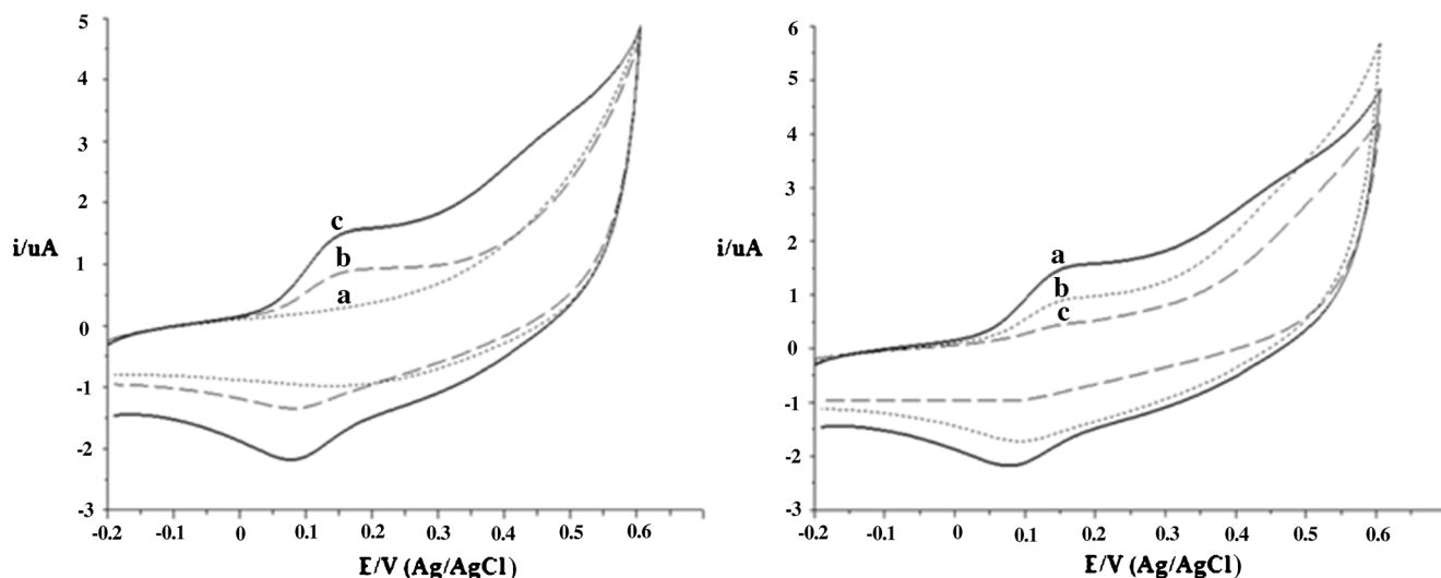
Fig. 4 (a) Cyclic-voltammetric behavior of (a) bare Au electrode, (b) Au-HDT (1 h), and (c) Au-HDT (1 h)-GNR; and of (b) (a) bare Au electrode, (b) Au-HDT (1 h)-GNR (1 h)-DNA probe, and (c) Au-
