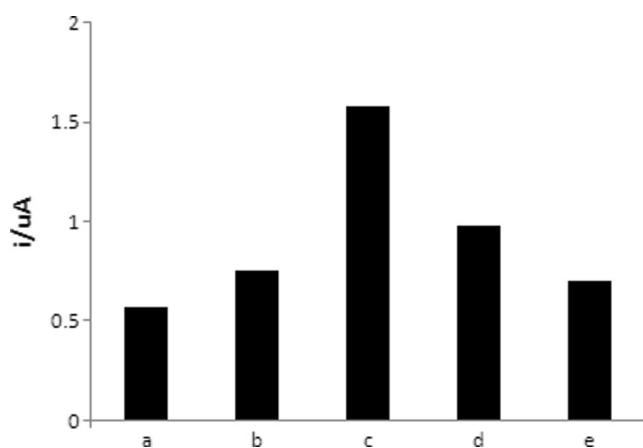
Fig. 5 Cyclic-voltammetric behavior of (a) bare Au electrode, (b) Au-HDT (1 h)-GNR (1 h)-DNA probe, (c) Au-HDT (1 h)-GNR (1 h)-DNA probe-DNA target (10 \mu\text{mol L}^{-1} ), (d) 10 \mu\text{mol L}^{-1} one-point-mismatch DNA, and (e) 10 \mu\text{mol L}^{-1} non-complementary DNA in 100 mmol L -1 buffer solution after incubation in 4 mmol L -1 [Co(phen) 3 ] 3+ for 1 h, at scan rate 50 mV s -1
