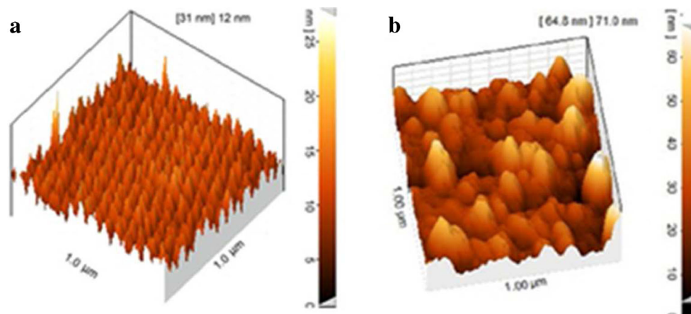
Fig. 3 AFM image of GNR-modified electrode before (a) and after (b) interaction with the DNA probe. The images were taken using semi-contact mode. Scan range was 1 \text{ } \mu\text{m} \times 1 \text{ } \mu\text{m}
