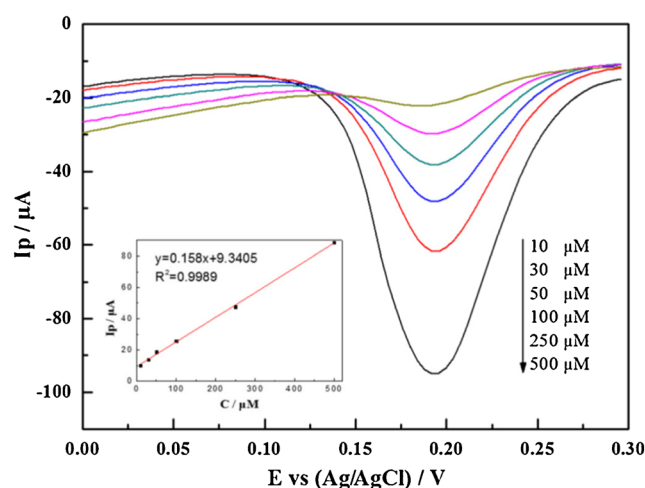
Fig. 14 Differential pulse voltammetric profiles of Ag-Pt-pECFs//GCE in the presence of different dopamine concentrations in nitrogen-saturated PBS. From top to bottom, the dopamine concentration is 10, 30, 50, 100, 250, 500 \mu\text{M} . Inset: the linear calibration curve. Reprinted with permission from Ref [40]. (Copyright American Chemical Society, 2014)
