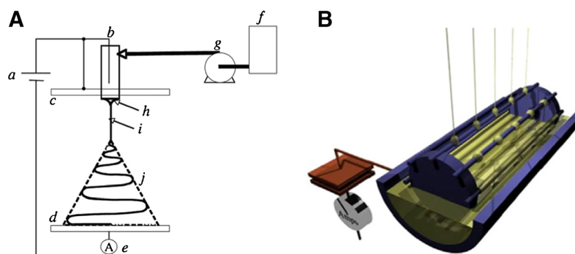
Fig. 1 (A) Schematic illustration of a conventional electrospinning set-up: (a) power supply (usually with high voltage capabilities up to 30 kV); (b) charging device; (c) electrode charged to a high potential (e.g., flat plate); (d) grounded electrode or collector (e.g., flat plate); (e) device for current measurements; (f) fluid reservoir; (g) flow rate control; (h) cone; (i) thinning jet; (j) whipping instability region. Reprinted with permission from Ref [32]. (Copyright Elsevier, 2007) (B) An example of free surface electrospinning. Conductive wires are used as the high voltage electrodes.
