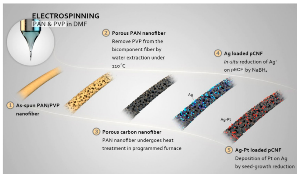
Fig. 12 Schematic illustration of the preparation of Ag-Pt-ECFs. Reprinted with permission from Ref [40]. (Copyright American Chemical Society, 2014)
