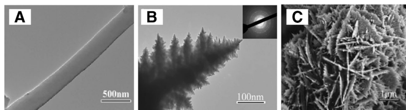
Fig. 17 TEM images of (A) ECF and (B) Pd-ECF. The inset in (B) shows the electron diffraction pattern of the TEM image. (C) SEM image of Pd-ECF prepared from a deposition potential of -0.2 V (versus Ag/AgCl)
