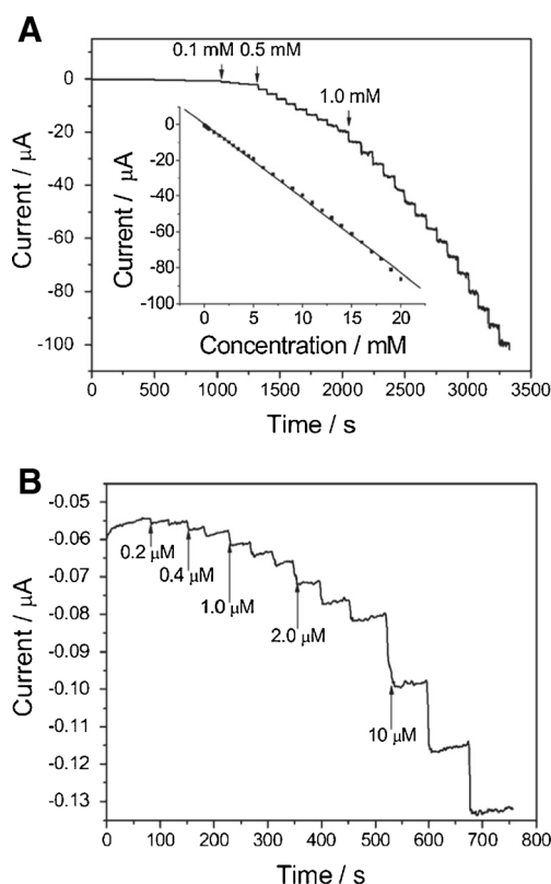
Fig. 9 (A) A representative chronoamperometric profile of Pd-ECF//CPE with successive addition of different concentrations of hydrogen peroxide into N_2 -saturated PBS (0.1 M, pH = 7.0). Inset: linear correlation between the current response and the H_2O_2 concentration between 0.2 \mu M and 20 mM. (B) The detailed current-time response of Pd-ECF//CPE at a fixed potential of 0.2 V (versus Ag/AgCl) in the presence of low concentrations of hydrogen peroxide. Reprinted with permission from Ref [97]. (Copyright John Wiley and Sons, 2008)
