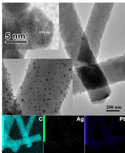
Fig. 13 TEM images of Ag-Pt-ECFs and the corresponding elemental mappings. Inset: high-resolution TEM of Ag-Pt bimetallic nanoparticles. Reprinted with permission from Ref [40]. (Copyright American Chemical Society, 2014)
