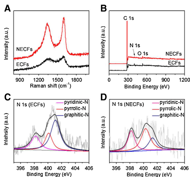
Fig. 6 (A) Raman spectra and (B) XPS survey scans of ECFs and N-ECFs. The high resolution N 1s spectra of (C) ECFs and (D) N-ECFs. Reprinted with permission from Ref [60]. (Copyright American Chemical Society, 2014)
