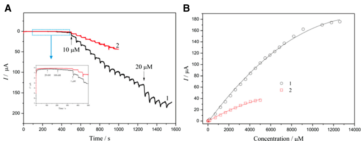
Fig. 11 (A) Current-time profiles of (1) PDA-Lac-Ni-ECF//MGCE and (2) PDA-Lac//MGCE at a fixed potential of 0.4V (versus Ag/AgCl) upon successive injection of catechol solutions into an acetate buffer solution. The inset shows an enlarged image of the data in the blue rectangle. (B)
