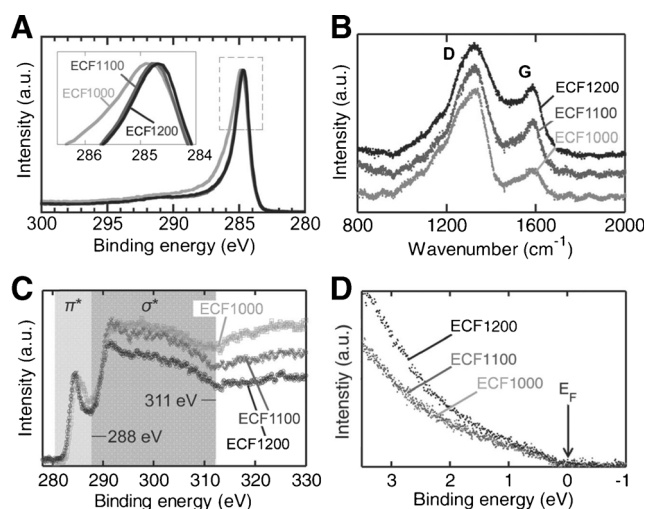
Fig. 4 Effect of carbonization temperature on the nanographite concentration and density of states for the ECF webs. (A) High resolution C 1 s spectra (inset: magnification of the dotted rectangular area). (B) Raman spectra. (C) EELS spectra. (D) UPS spectra showing the density of electronic states near the Fermi level. Reprinted with permission from Ref [51]. (Copyright John Wiley and Sons, 2013)
