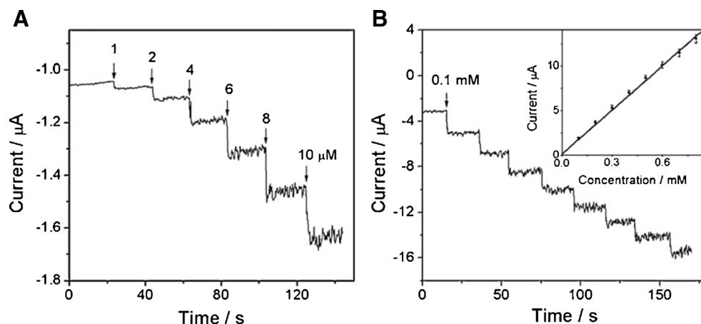
Fig. 16 A representative chronoamperometric profile of the Pt-ECF electrode at a fixed potential of 0 V (versus Ag/AgCl) with successive injection of hydrogen peroxide at (A) low concentrations and (B) 0.1 mM. Inset of (B) shows the linear relationship between the current and the \text{H}_2\text{O}_2 concentration. Reprinted with permission from Ref [109]. (Copyright Elsevier, 2011)
