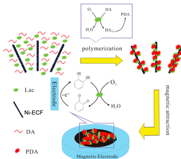
Fig. 10 Schematic illustration of the fabrication processes of PDA-Lac-Ni-ECF composites and the resulting sensors. Reprinted with permission from Ref [106]. (Copyright American Chemical Society, 2014)
