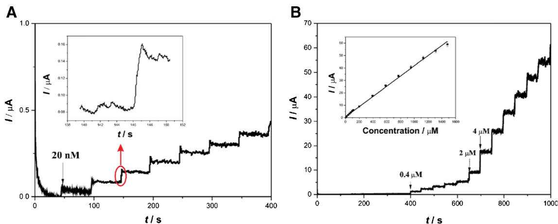
Fig. 5 (A) A representative chronoamperometric profile (up to 400 s) of laccase/Nafion/ECFs//GCE when catechol solutions were added to an acetate buffer solution under constant stirring. Inset: enlarged red circle showing the third addition of catechol. (B) The chronoamperometric
