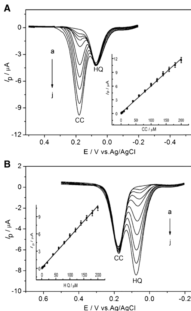
Fig. 3 DPVs for ECF-CPE in (A) different concentrations (a–j: 1, 2, 5, 10, 40, 80, 120, 160, 200 \mu\text{M} ) of CC containing 50 \mu\text{M} HQ and (B) different concentrations (a–j: 1, 2, 5, 10, 40, 80, 120, 160, 200 \mu\text{M} ) of HQ containing 50 \mu\text{M} CC. Insets show the calibration plots of CC and HQ. Reprinted with permission from Ref [38]. (Copyright Elsevier, 2012)
