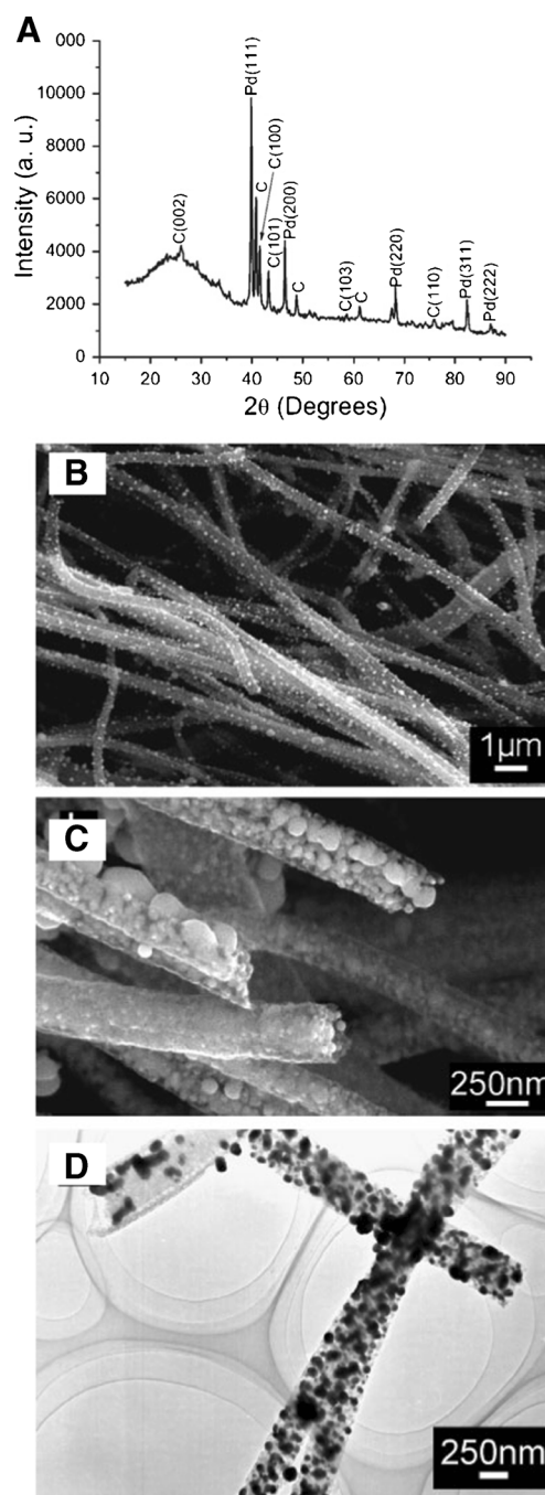
Fig. 8 (A) XRD pattern, (B) SEM image, (C) high magnification SEM image, and (D) TEM image of Pd-ECF nanocomposites. Reprinted with permission from Ref [97]. (Copyright John Wiley and Sons, 2008)
