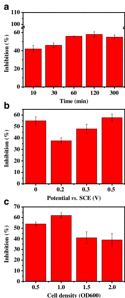
Fig. 2 The effect of (a) preincubation time (working electrode potential set at 0.5 V, the cell density is OD 600 = 0.5), (b) poised potential (preincubation with DCP for 60 min, the cell density is OD 600 = 0.5), and (c) cell density (preincubation with DCP for 60 min, working electrode potential set at 0.5 V) on the performance of the developed biosensor (DCP, 20 mg/L). The amperometric response from cells without DCP addition at designed condition was used as the control for inhibition ratio calculation
