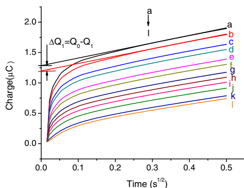
Fig. 5 Chronocoulometric curves in 50 mM RuHex for the prepared electrochemical biosensor in the presence of various concentrations of \text{Pb}^{2+} : a 0 nM; b 0.01 nM; c 0.05 nM; d 0.1 nM; e 0.5 nM; f 1 nM; g 5 nM; h 10 nM; i 20 nM; j 50 nM; k 100 nM; l 200 nM
