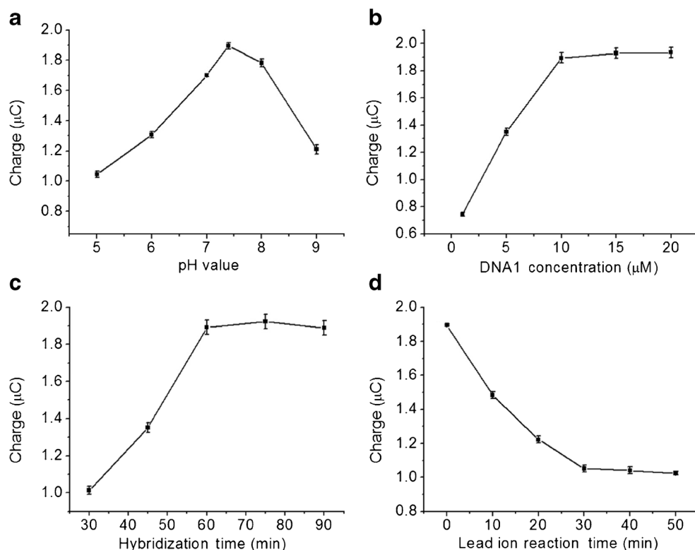
Fig. 4a–d Influences of a the pH value, b the DNA1 concentration, c the hybridization time, and d the \text{Pb}^{2+} reaction time (lead ion concentration: 70 nM) on the CC response signal
