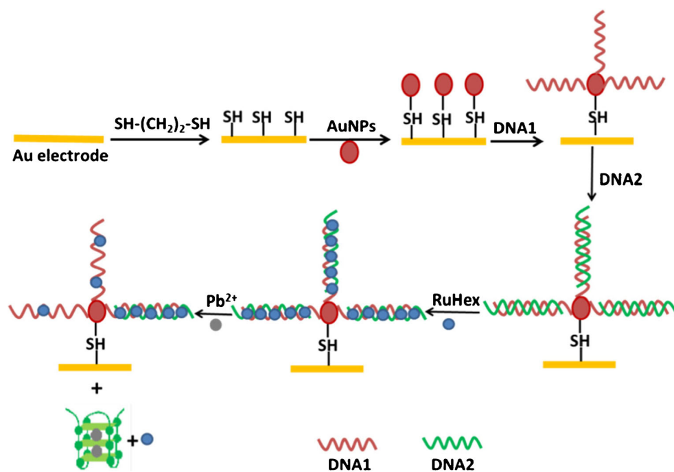
Scheme 1 Description of the \text{Pb}^{2+} detection strategy
