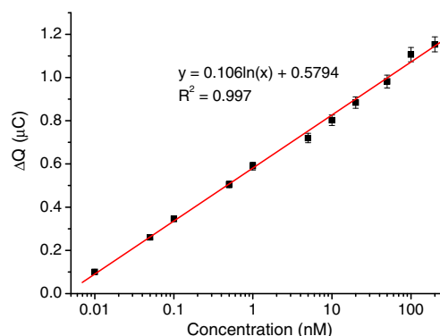
Fig. 6 Calibration curve for \text{Pb}^{2+} concentration (0.01–200 nM)
