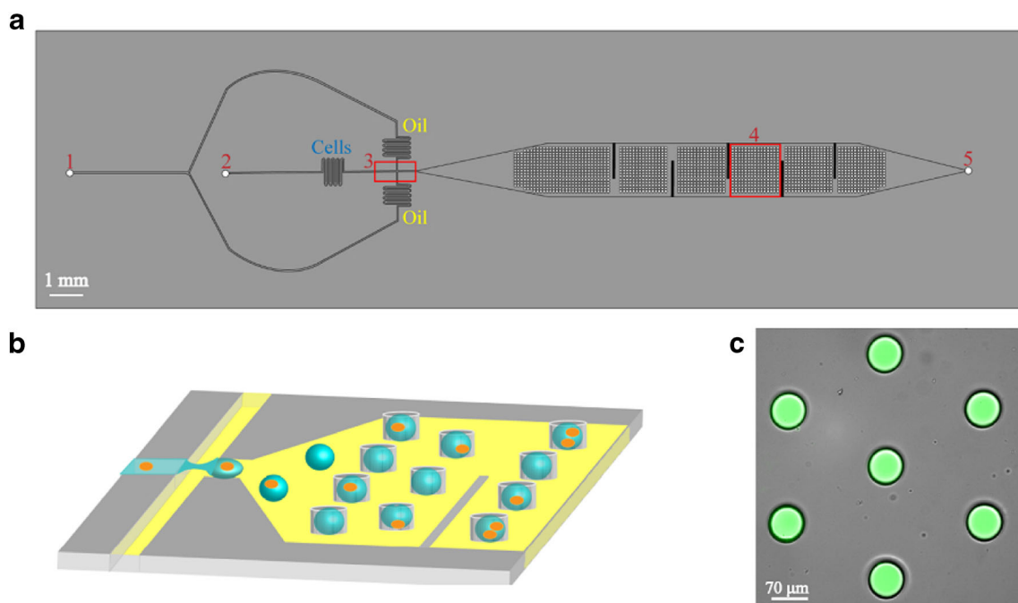
Fig. 1 Schematic of the microfluidic droplet trapping platform. a Top view of the device illustrating the (1) oil inlet, (2) water inlet, (3) flow-focusing junction, (4) droplet trapping array, and (5) outlet. b Schematic of the generation and trapping of droplets containing cells into 70- \mu\text{m}
