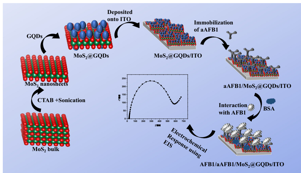
Fig. 1 Schematic illustrations of electrochemical biosensor for aflatoxin B1 detection using \text{MoS}_2\text{@GQD} composite
