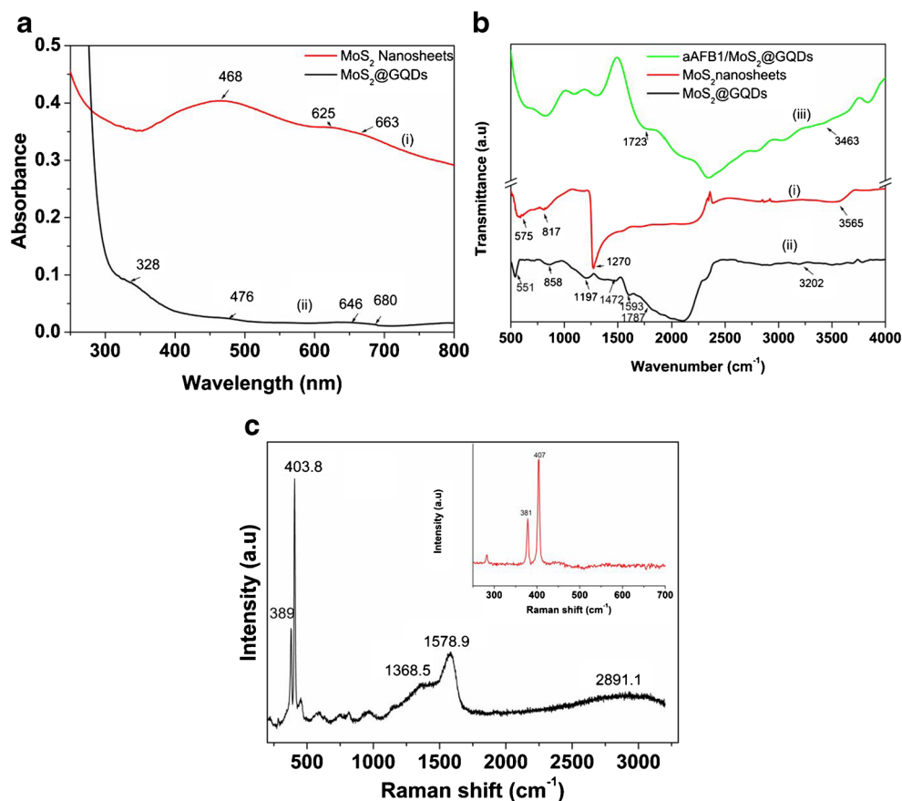
Fig. 2 a UV-vis absorbance spectrum of (i) MoS 2 nanosheets and (ii) MoS 2 @GQD composite in aqueous medium. b FT-IR of (i) MoS 2 /ITO, (ii) MoS 2 @GQDs/ITO composite, and (iii) biomolecule immobilized electrode aAFB1/MoS 2 @GQDs/ITO. c Raman spectrum of MoS 2 @GQDs (inset image: Raman spectrum of MoS 2 )
