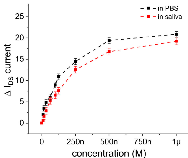
Fig. 5 Sensing characteristics of gFET for HPV-16 E7 proteins. Calibration curve of the HPV-16 E7 protein sensor in PBS (black) and in saliva (red). Protein sensing in real time using aptamer-modified rGO-FET when the device is exposed to increasing concentrations of HPV-16 E7 proteins (7.5, 15, 31, 62, 100, 125, 250, 500, and 1000 nM)
