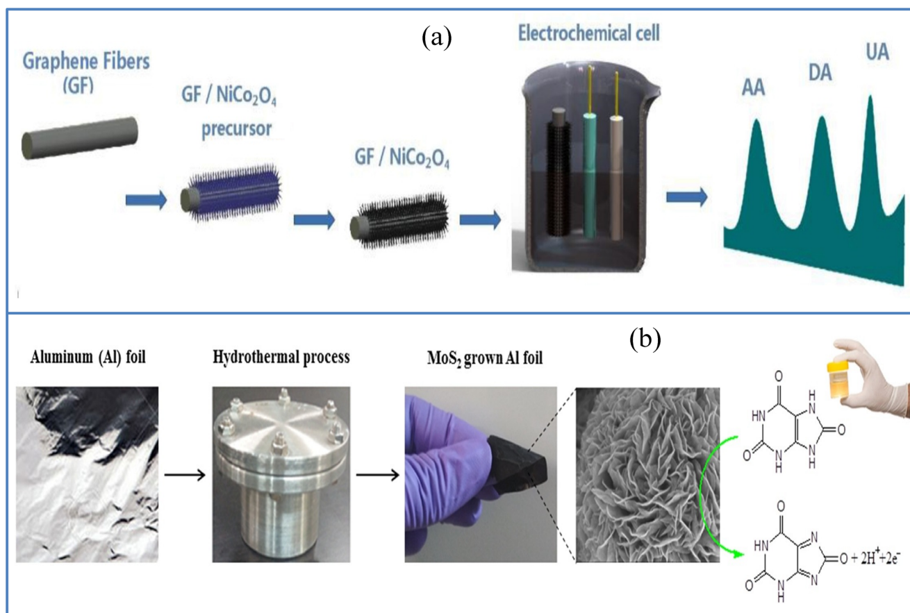
Fig. 5 Flexible as well as a wearable sensor for detection of small molecules like ascorbic acid, uric acid, and so on. a Fiber-based \text{GF} / \text{NiCo}_2\text{O}_4 sensor for the detection of AA, DA, and UA (source: reprinted from Weihua Cai, Jianwei Lai, Ting Lai, Haoting Xie, Jianshan Ye-Controlled functionalization of flexible graphene fibers for the simultaneous determination of ascorbic acid, dopamine and uric acid, Sensors and Actuators B: Chemical , 224 (2016)225–232, with permission from
