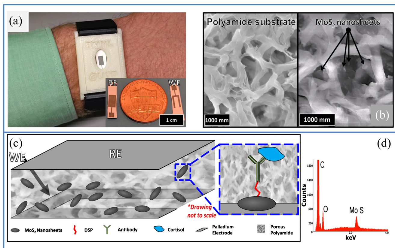
Fig. 18 a Illustration for the presumed cortisol transdermal sweat monitoring prototype device. b SEM images of polyamide substrate before and after MoS 2 coating. c Schematic representation of the prepared MoS 2 -based cortisol sensor d EDAX spectra. Source: Kinnamon, David, Ghanta, Ramesh Lin, Kai Chun Muthukumar,
