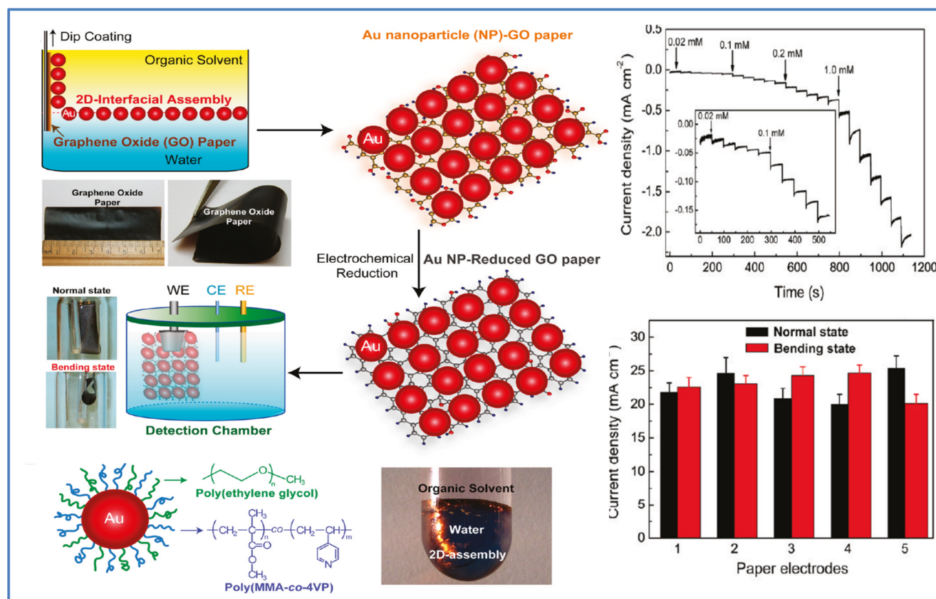
Fig. 8 Two-dimensional material-based flexible/wearable sensor for \text{H}_2\text{O}_2 detection. Diagrammatic representation of fabrication \text{H}_2\text{O}_2 sensor based on the hybrid electrode of 2D Au particles on graphene paper and corresponding amperometric response of the fabricated sensor (source: reprinted from Fei Xiao, Jibin Song, Hongcai Gao, Xiaoli Zan, Rong Xu,
