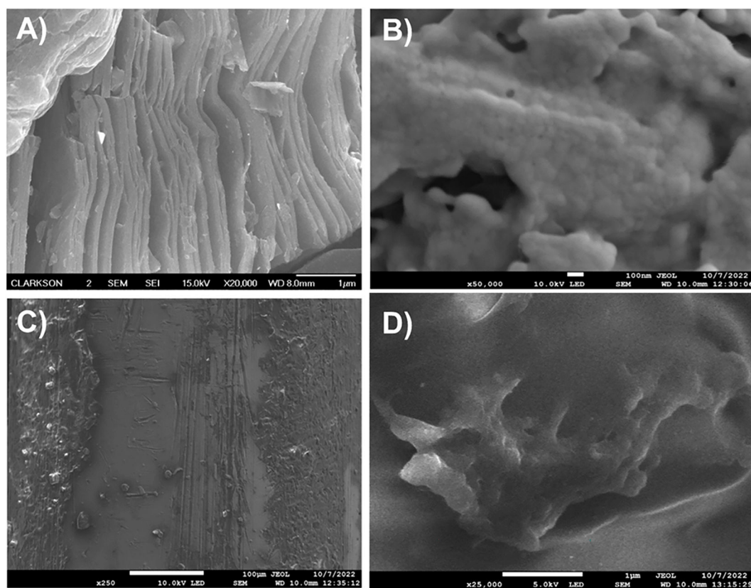
Figure 2. SEM images of MXene (A), Sensor surface after cleaning (B) Sensor surface after superoxide dismutase immobilization step (C), and sensor surface after MXene deposition step (D). Scale bar A-1μm, B-100nm, C-100μm and D-1μm.
