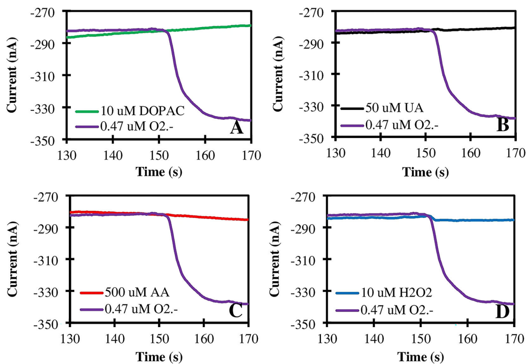
Figure 5. Sensor response to 10 \mu\text{M} DOPAC (A), 50 \mu\text{M} UA (B), 500 \mu\text{M} AA (C), or 10 \mu\text{M} \text{H}_2\text{O}_2 (D) measured in 0.1M PBS, pH 7.5.
