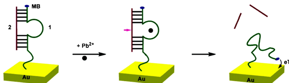
Fig. 6 A schematic of the DNAzyme-based electrochemical sensor [70]. Copyright 2007, ACS Publications
