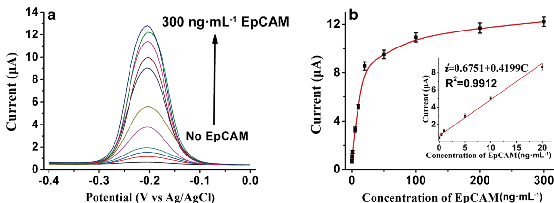
Fig. 2 a Typical SWV current response of the modified electrode to different concentrations of EpCAM in the presence of EpCAM aptamer/probe A and Hp2 (from bottom to top: 0 to 300 \text{ng}\cdot\text{mL}^{-1} ); b The relationship curve of SWV current responses vs. the concentrations of EpCAM from 0 to 300 \text{ng}\cdot\text{mL}^{-1} . Inset of (b): linear relationship
