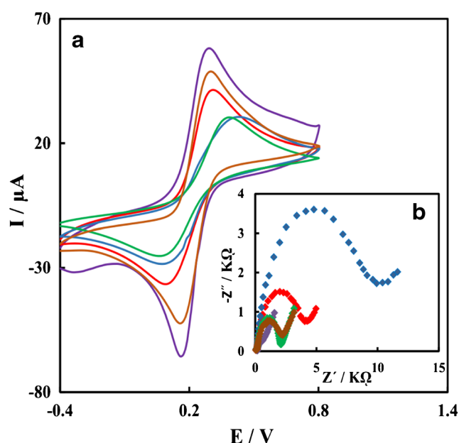
Fig. 5 a Cyclic voltammograms and (b) Nyquist plots of GCE (green line), \text{GCE/MWCNT/Fe}_3\text{O}_4\text{-SH@Au} (purple line), \text{GCE/MWCNT/Fe}_3\text{O}_4\text{-SH@Au/aptamer} (brown line), \text{GCE/MWCNT/Fe}_3\text{O}_4\text{-SH@Au/aptamer/MCH} (red line) and \text{GCE/MWCNT/Fe}_3\text{O}_4\text{-SH@Au/aptamer/MCH/BPA} (blue line) in 5 mM \text{Fe}(\text{CN})_6^{3-/4-} (1:1) solution containing 0.1 M KCl at Scan rate 0.1 \text{ V s}^{-1}
