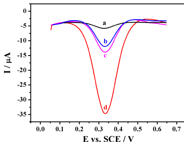
Fig. 3 DPV curves of different electrodes: without DNA-linked AuNPs composite (a), without SA-ALP (b), without TB (c), SA-ALP/DNA-linked \text{AuNPs}/\text{TB}/\text{MCH}/\text{TBA1}/\text{AuNPs}/\text{WSe}_2/\text{GCE} (d)
