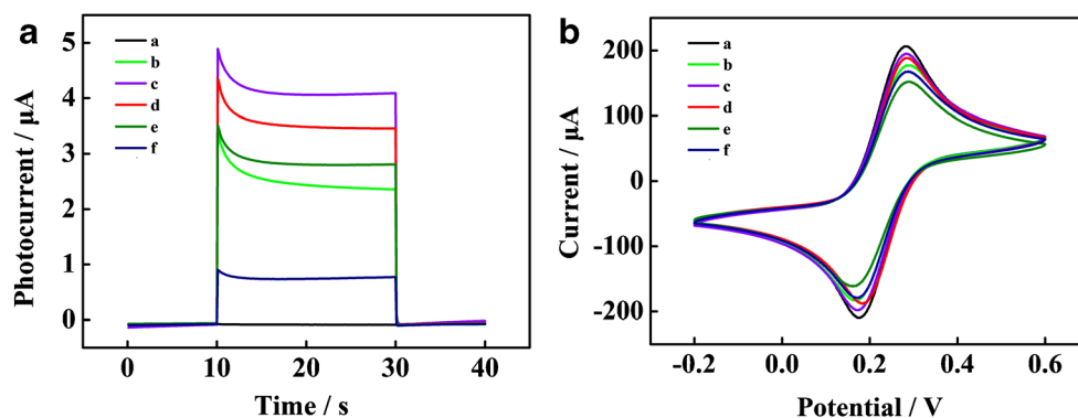
Fig. 3 a PEC responses of (a) GCE, (b) g-C 3 N 4 /GCE, (c) AuNPs/g-C 3 N 4 /GCE, (d) S 0 /AuNPs/g-C 3 N 4 /GCE, (e) HT/S 0 /AuNPs/g-C 3 N 4 /GCE, (f) S 1 -carbon/target VEGF 165 /HT/S 0 /AuNPs/g-C 3 N 4 /GCE with 365 nm irradiation in 0.1 M pH 7.0 PBS containing 0.1 M H 2 O 2 . (b) CV responses of (a) GCE, (b) g-C 3 N 4 /GCE, (c) AuNPs/g-C 3 N 4 /GCE, (d)
