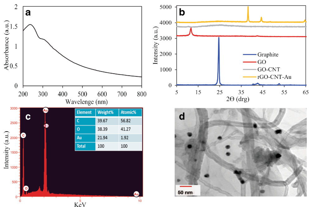
Fig. 1 Characterization of the nanocomposite a UV-Vis absorption spectrum of the GO nano-sheets b The XRD images of graphite, GO, GO-CNT hybrid and the rGO-CNT-Au nanocomposite c The EDX spectra of the rGO-CNT-Au nanocomposite d The TEM micrograph of the rGO-CNT-Au nanocomposite
