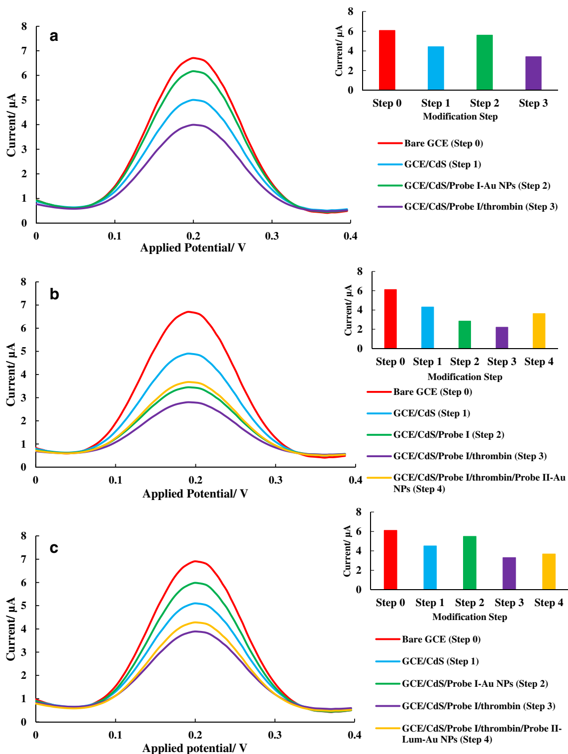
Fig. 1 The DPV curves of the biosensor in a QM, b AM, and c RM at different preparation steps in PBS (0.1 M, pH = 7.5) containing 5 mM K_4[Fe(CN)_6] , K_3[Fe(CN)_6] and 0.1 M KCl at scan rate of 100 \text{ mV.s}^{-1} (Insets: The peak current versus preparation steps)
