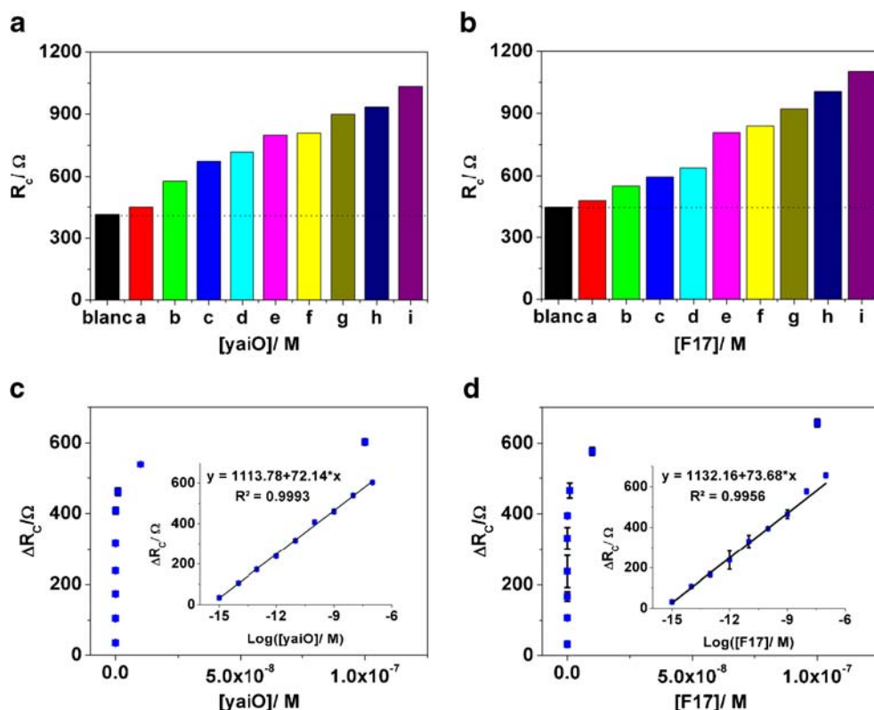
Fig. 2 The value of R_{ct} obtained after detection of various yaiO (a) and fli7 (b) concentrations: (a) 10^{-15} M; (b) 10^{-14} M; (c) 10^{-13} M; (d) 10^{-12} M; (e) 10^{-11} M; (f) 10^{-10} M; (g) 10^{-9} M; (h) 10^{-8} M; and (i) 10^{-7} M; c and d are related to the calibration curves of \Delta R_{ct} vs. [yaiO] and [fli7] , respectively; Inset: representations of \Delta R_{ct} vs. \log [yaiO] and \log [fli7] , respectively. Error bars, SD, n = 3
