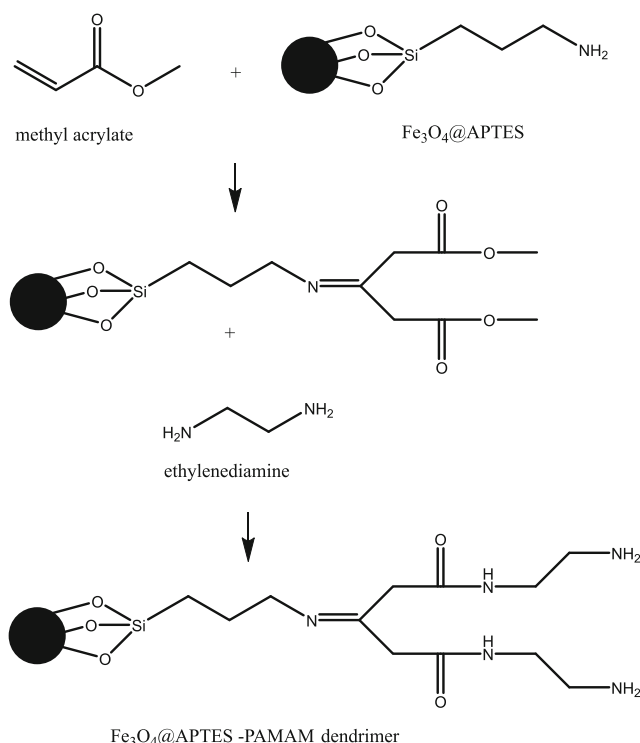
Scheme 1 PAMAM dendrimer formation at APTES-functionalized Fe 3 O 4 core. Coupling of terminal amine groups with glutaraldehyde subsequently enabled enzyme attachment
