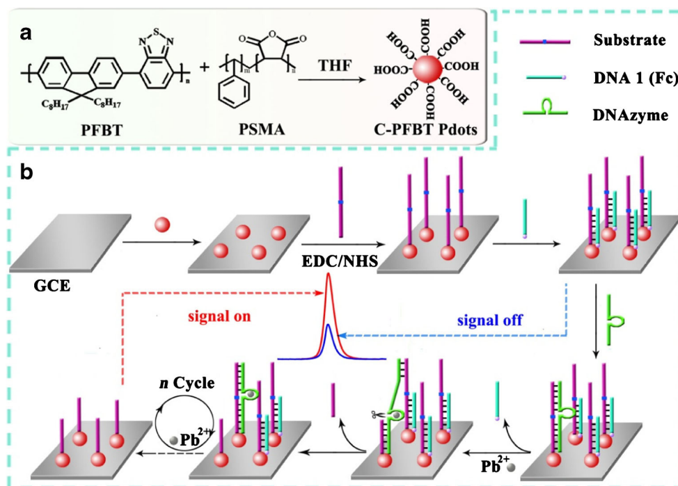
Scheme 1 Schematic illustration of a the preparation of C-PFBT Pdts and b the fabrication of the biosensor
