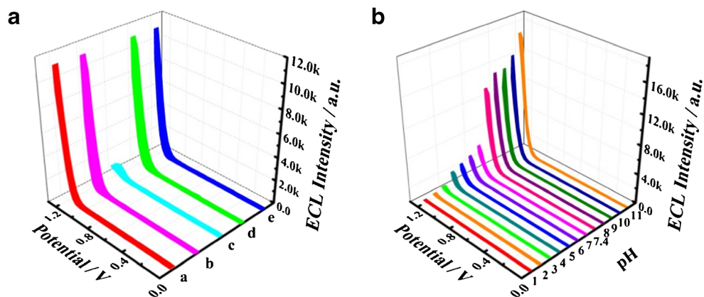
Fig. 2 a The ECL response of C-PFBT Pdts/GCE in PBS (0.10 M pH 7.4) with (a) air-saturated and (b) \text{N}_2 -saturated, (c) in MeCN solution under air-saturated, in PBS (0.10 M pH 7.4) containing (d) L-cys and (e) SOD. b ECL response of C-PFBT Pdts/GCE in PBS (0.10 M pH 7.4) with pH from 1 to 11. Scanning potential range, 0–1.25 V; scanning rate, 300 mV/s
