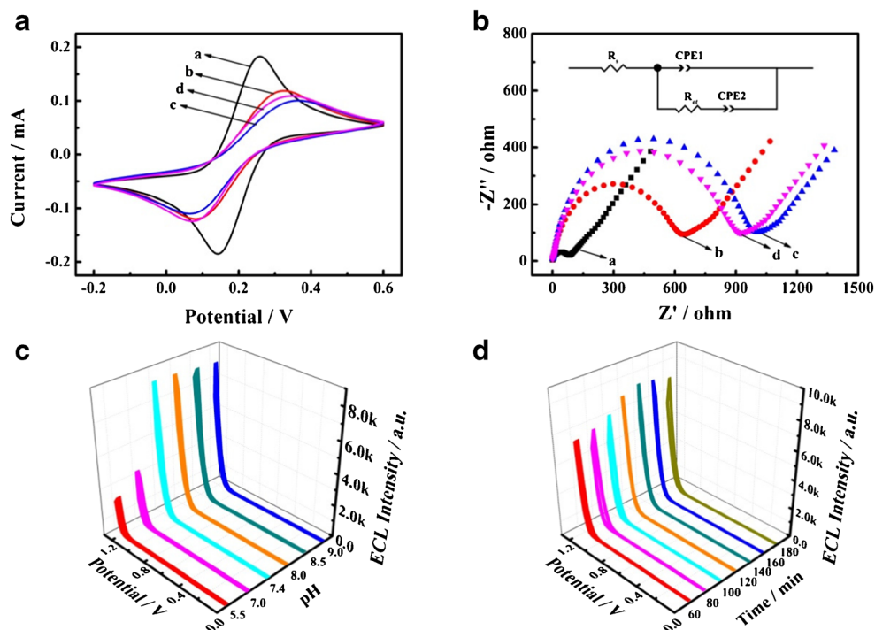
Fig. 3 a CV and b EIS diagrams of (a) bare GCE, (b) C-PFBT Pdots/GCE, (c) C-PFBT Pdots/GCE with substrate and Fc-labeled DNA 1, (d) C-PFBT Pdots/GCE with substrate, DNAzyme and \text{Pb}^{2+} in 5.0 mM [\text{Fe}(\text{CN})_6]^{3-/4-} solution. The insert of b: the equivalent circuit. The effect of c pH of PBS solution and d incubation time of \text{Pb}^{2+} on the ECL response at the biosensor. Scanning potential range of -0.2 – 0.6 V and scanning rate of 100 mV/s for CV detection. The init potential of 0.22 V, amplitude of 5 mV, and frequency of 0.1 – 10^5 Hz for EIS detection. Scanning potential range of 0 – 1.25 V and scanning rate of 300 mV/s for ECL detection
