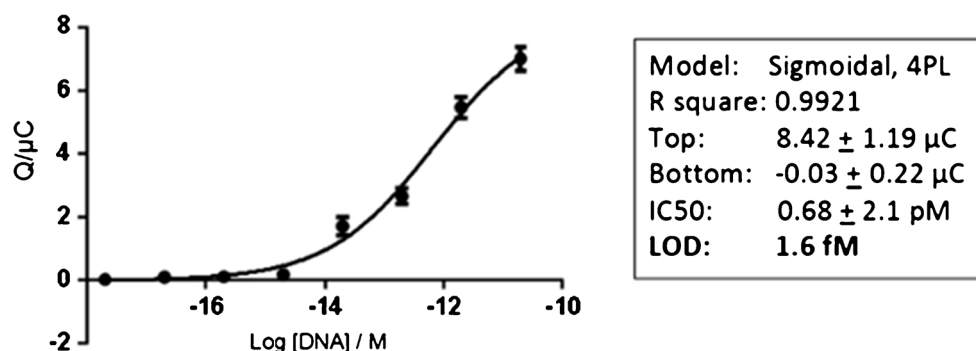
Fig. 6 Calibration plot obtained by amplifying a range of concentrations (20 pM to 20 aM) of dsDNA template starting concentrations after 40 min RPA and 10 min hybridization with capture probe and 10 min hybridization with reporter probe
