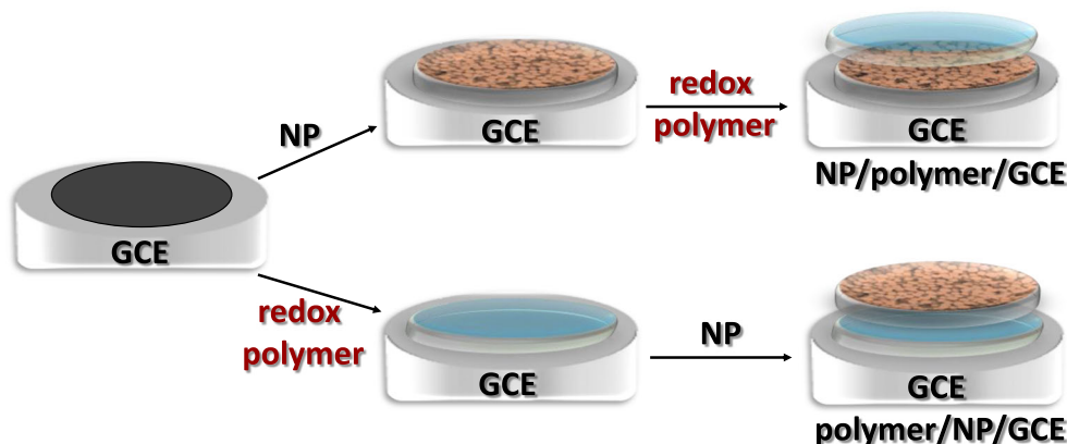
Fig. 6 The fabrication steps of NP/polymer and polymer/NP-modified glassy carbon electrodes
