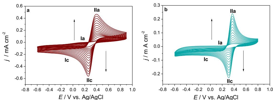
Fig. 7 Potential cycling electropolymerization on \text{Fe}_2\text{O}_3/\text{GCE} in ethaline DES / 1.0 M \text{H}_2\text{SO}_4 , scan rate 50 \text{ mV s}^{-1} of a 1 mM NR to form \text{PNR}_{\text{Ethaline}} and b 1 mM MG to form \text{PMG}_{\text{Ethaline}} . Adapted from [66], reprinted by permission of Elsevier
