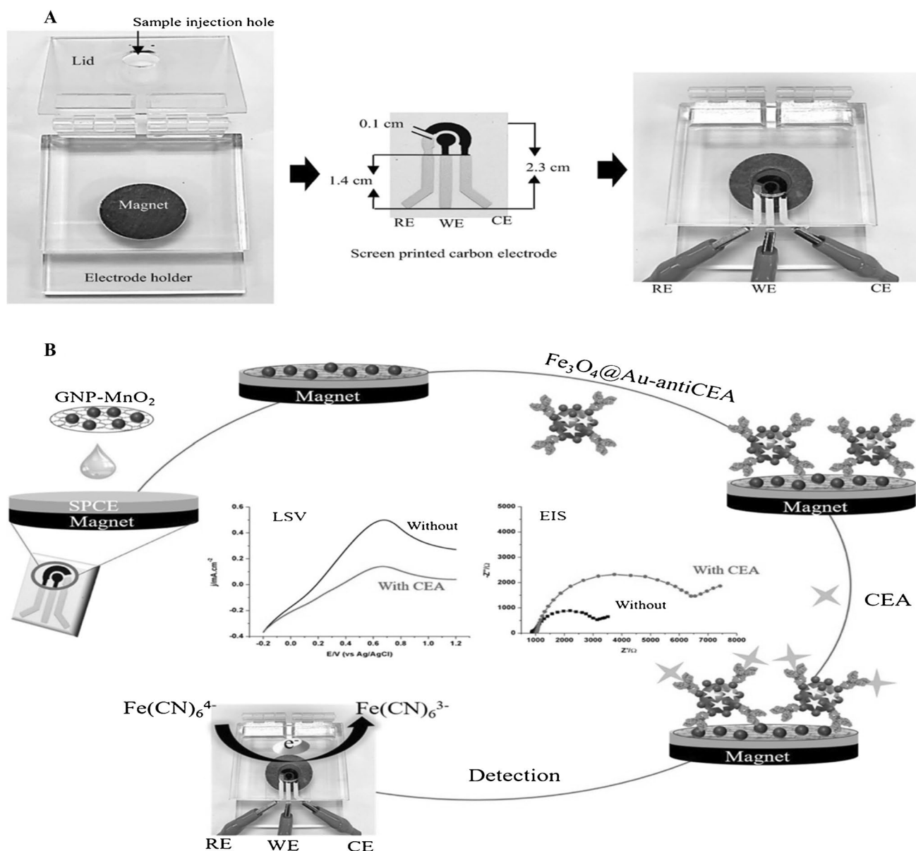
Fig. 6 A The electrode holder set-up and SPCE, (B) schematic demonstration of the electrochemical sensor fabrication steps for detection of CEA.4P. Reprinted from Ref. [43] with permission from Elsevier
