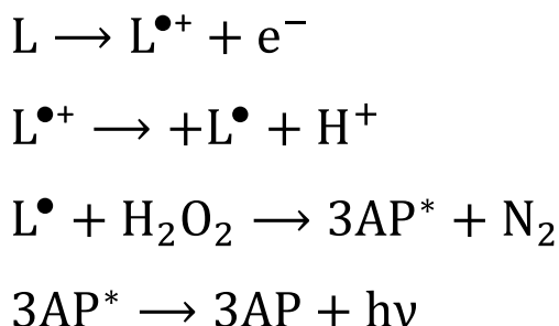
Scheme 6 Simplified reaction mechanism for ECL of luminol (L) with H_2O_2
