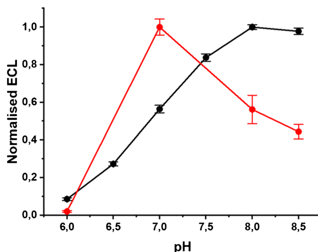
Fig. 5 Normalized ECL as a function of pH: \text{Ru}(\text{bpy})_3^{2+} free diffusing in solution (black), and \text{Ru}(\text{bpy})_3^{2+} labeled on 2.8- \mu\text{m} beads deposited on the electrode (red). Adapted with permission from [51], Copyright (2023) Royal Society of Chemistry
