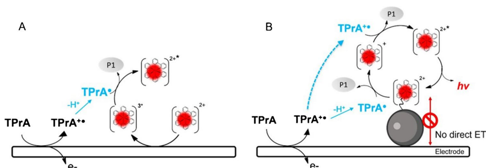
Fig. 4 Schematic representation of electrogenerated chemiluminescence mechanism involving TPrA and \text{Ru}(\text{bpy})_3^{2+} :
