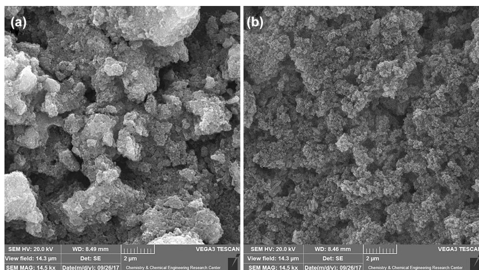
Fig. 2 Scanning electron microscopy of a bare MNPs and b Ty-Cyc/EMNPs
