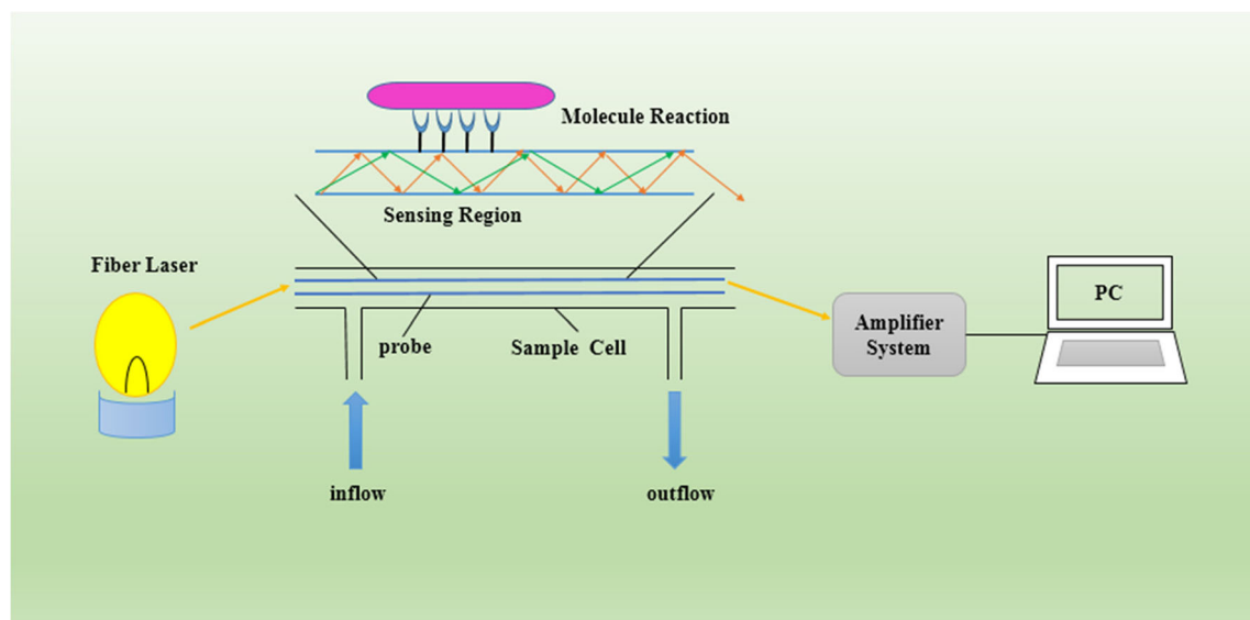
Fig. 2 The schematic representation of fiber-optic biosensors
