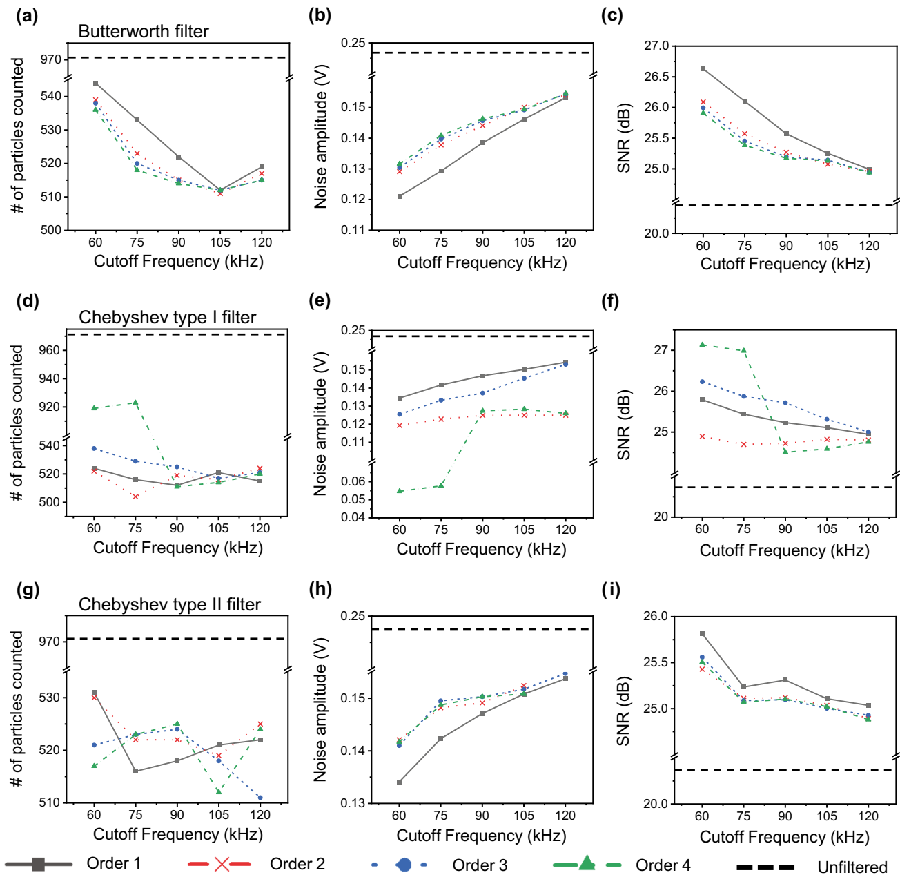
Fig. 4 Low pass filtering results when varying the cutoff frequency (60 kHz to 120 kHz) with different filter types (Butterworth (a–c), Chebyshev Type I (d–f), Chebyshev Type II (g–i) filter types) and different filter orders: 1 st order (gray), 2 nd order (red), 3 rd order (blue), 4 th order (green). Results compared with the number of particles counted through the impedance detection recording (a, d, g), the
