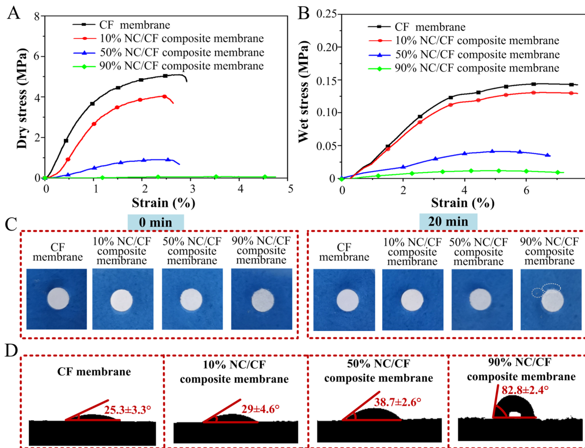
Fig. 3 The physical properties of these pure CF membranes and NC/CF composite membranes. A The dry tensile strength of these pure CF membranes and NC/CF composite membranes. B The wet tensile strength of these pure CF membranes
