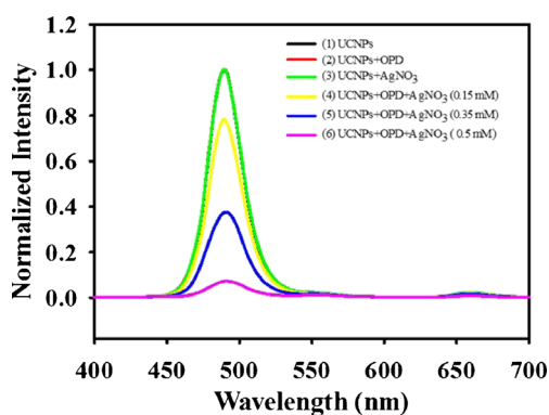
Fig. 2 Fluorescence spectra of UCNPs solution. (1) only UCNPs, (2) UCNPs + OPD, (3) UCNPs + \text{AgNO}_3 , (4) UCNPs + OPD + \text{AgNO}_3 (0.15 mM), (5) UCNPs + OPD + \text{AgNO}_3 (0.35 mM), (6) UCNPs + OPD + \text{AgNO}_3 (0.5 mM), respectively. [UCNPs]: 0.1 mg/mL. [OPD]: 1 mM
