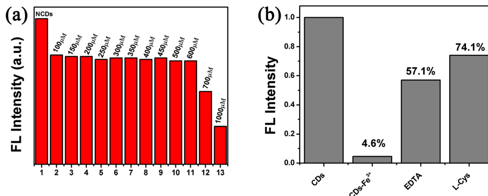
Fig. 2 a The fluorescence intensity of the NCDs with the different concentrations of \text{Fe}^{3+} ions, and then L-Cys (1 mM) was added. b The fluorescence intensity of the NCDs, NCDs- \text{Fe}^{3+} , NCDs- \text{Fe}^{3+} -EDTA, NCDs- \text{Fe}^{3+} -L-Cys
