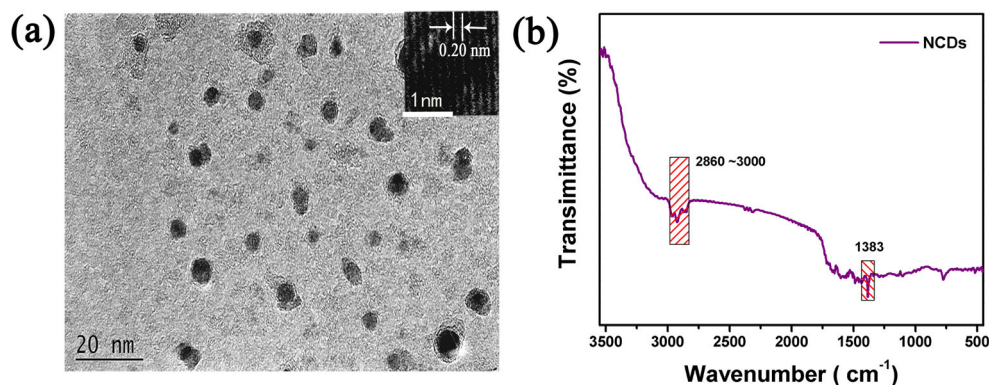
Fig. 1 a TEM images, b FT-IR spectra of NCDs and precursors. Inset in (a) : the lattice fringes of NCDs from HRTEM observation
