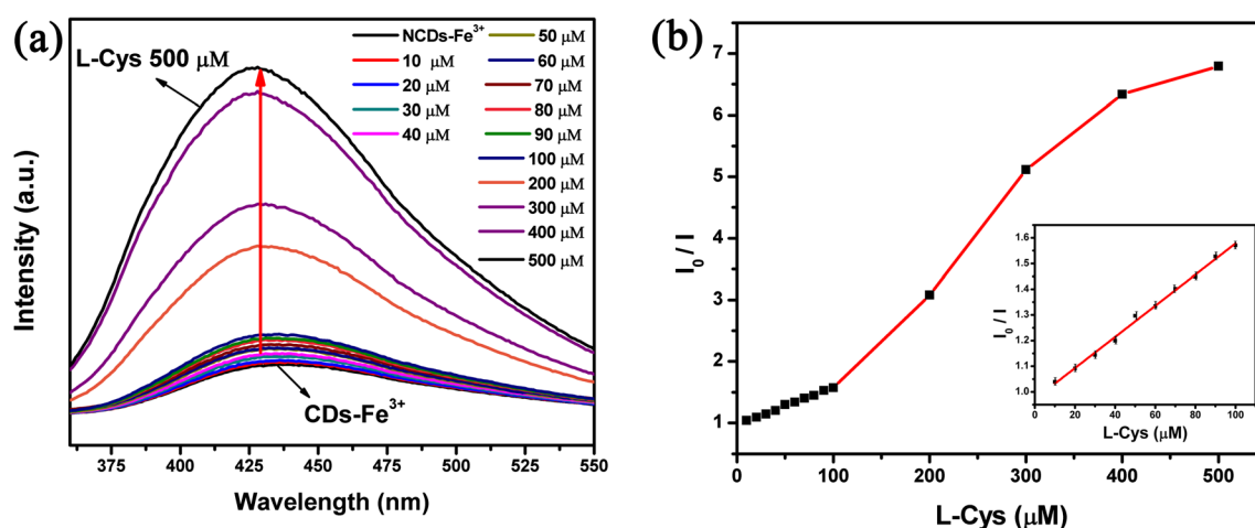
Fig. 3 a Fluorescence titration curve of the NCDs - \text{Fe}^{3+} with concentrations of L-Cys ions from 0 to 500 \mu\text{M} . b PL emission change of NCDs with different concentrations of L-Cys, where I and I_0 are the
