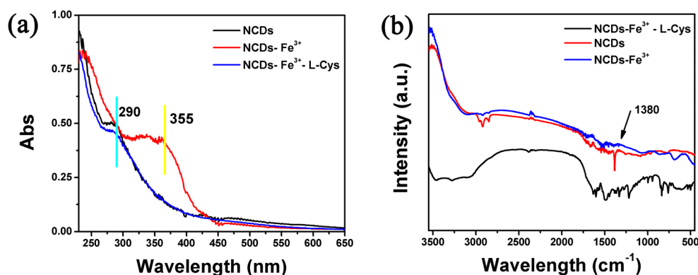
Fig. 4 UV-vis absorption spectrum of the NCDs, NCDs- \text{Fe}^{3+} and NCDs- \text{Fe}^{3+} -L-Cys (a). FT-IR spectra of NCDs, NCDs- \text{Fe}^{3+} and NCDs- \text{Fe}^{3+} -L-Cys (b)
