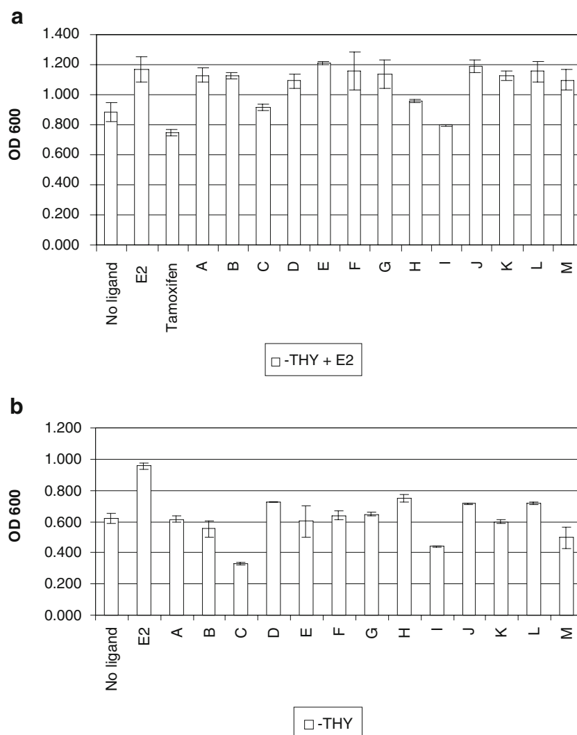
Fig. 4. (a) Cell growth as determined by OD 600 of E. coli D1210 \Delta thyA cells transformed with pMIT::ER \alpha * and grown in -Thy medium with 10 \mu M E2 at 34°C for 13 h in the presence of the test ligands. The concentration of all of the ligands was 10 \mu M except of tamoxifen, which had a concentration of 2 \mu M. (b) Cell growth as determined by optical density [OD 600] of E. coli D1210 \Delta thyA cells transformed with pMIT::ER \alpha * and grown in -Thy medium at 34°C for 13 h. The concentration of all compounds was 10 \mu M. Experiments were performed in triplicate and error bars represent one standard deviation.
