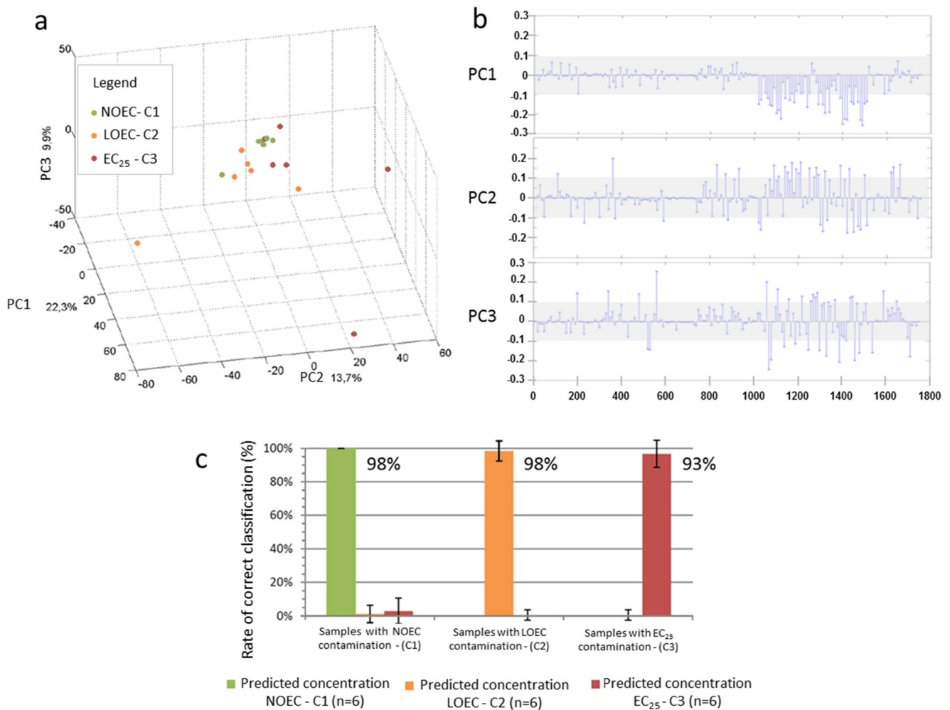
Fig. 2 Principal component analysis of synthetic samples based on the global panel of 1870 transcriptomic reporters according to their metallic contamination (A) and the associated loadings presenting the contribution to the first 3 axes of the PCA. The shaded space corresponds to the pool of
