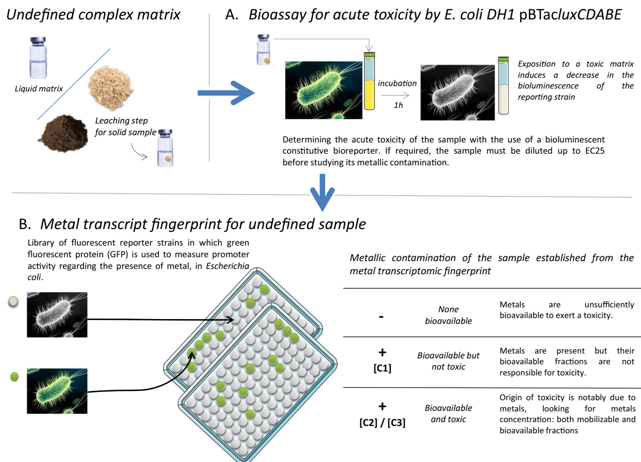
Fig. 4 Schematic role of the testing procedure in the characterization of unknown complex samples
