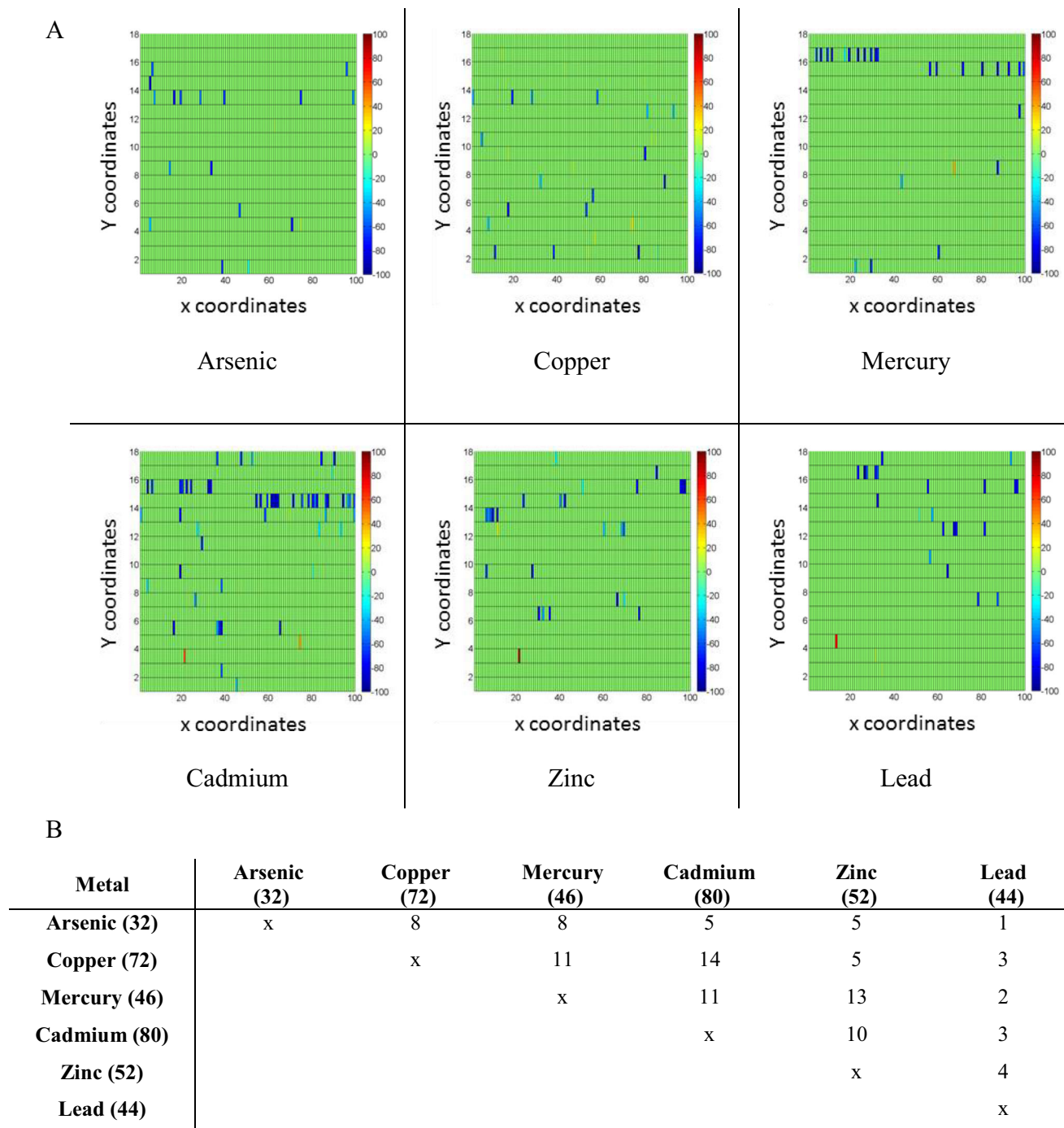
Fig. 1 Transcriptomic regulation in response to metals at the C2 concentrations. A Transcriptomic fingerprints induced by the presence of the dedicated metal with IndRF values of [-100, 0] for repressed transcripts, 0 for unregulated transcripts and [0, 100] for activated
