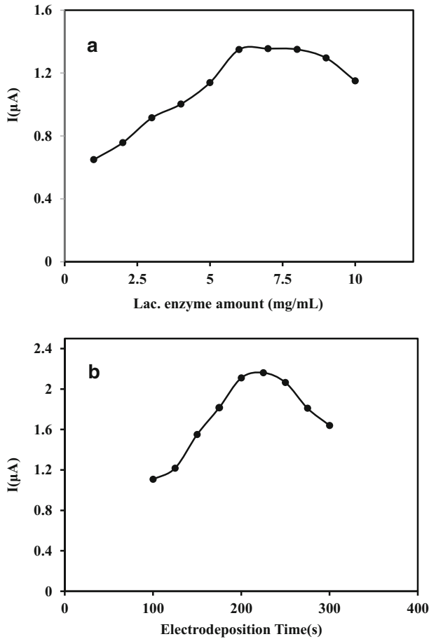
Fig. 4 Amperometric response of biosensor for catechol by varying of a ) amount of the Lac enzyme and b ) electrodeposition time in PBS (0.05 M, pH=7) containing 30 \mu M catechol
