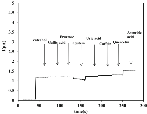
Fig. 7 Amperometric response of the \text{Fe}_3\text{O}_4/\text{PANI}/\text{Lac}/\text{CS}/\text{CPE} toward 10\ \mu\text{M} catechol upon addition of interferents of uric acid, ascorbic acid, gallic acid, cysteine, quercetin, and caffeine at a 100\ \mu\text{M} concentration level
