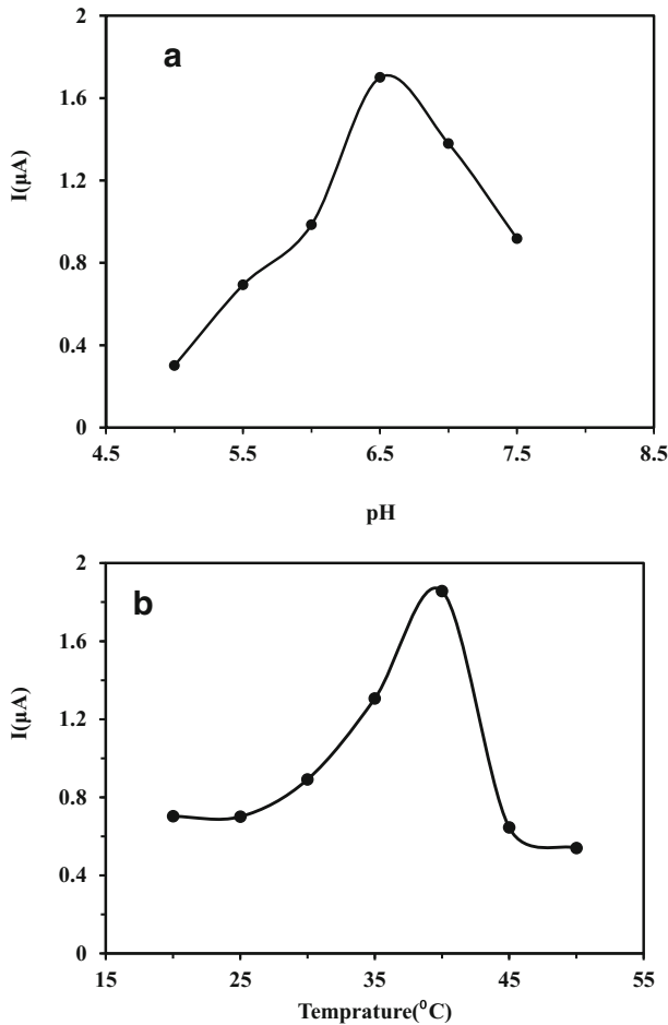
Fig. 5 Effect of a pH and b temperature on the response of the biosensor toward 200 μM catechol in PBS at +0.2 V vs. Ag/AgCl
