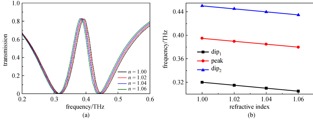
Fig. 5 (a) Spectral transmission at different refractive indices; (b) resonance frequency of dip_1 /peak/ dip_2 versus the refractive index
