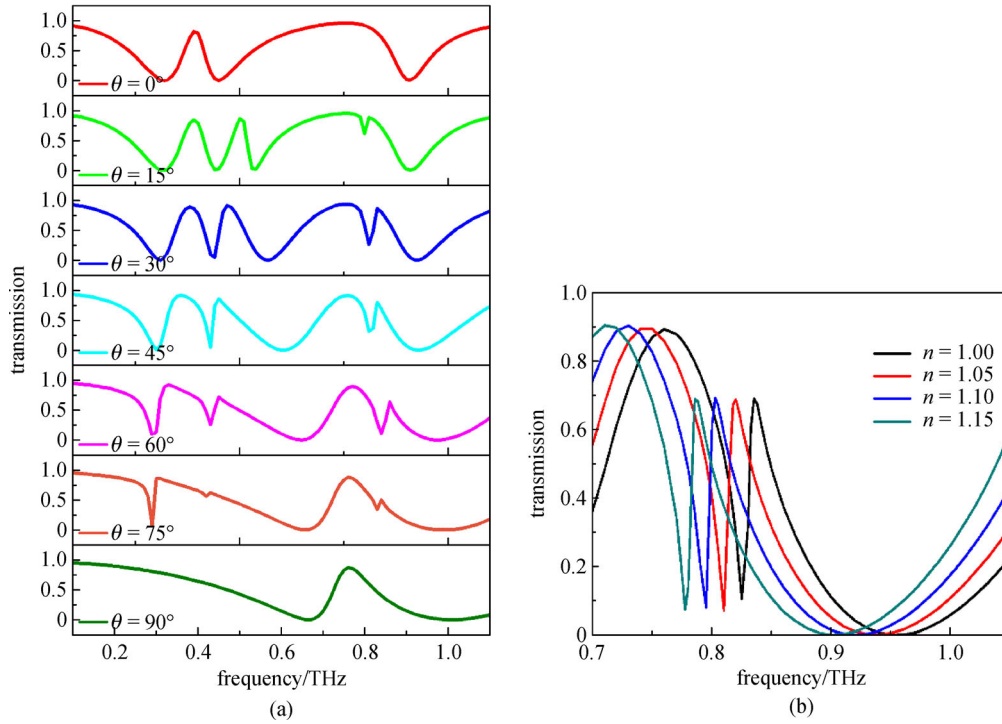
Fig. 6 (a) Transmission spectrum under different polarizations; (b) transmission spectra at different refractive indices. The polarization angle \theta = 60^\circ
