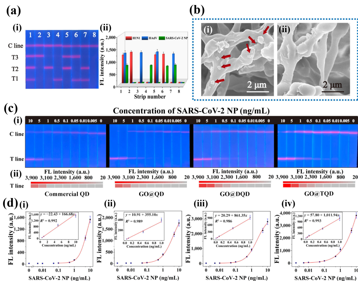
Figure 3 (a)(i) Images and (ii) corresponding fluorescence intensities of GO@TQD-based LFA for evaluating the cross-reactivity of three target respiratory viruses. (b) Typical SEM images of the test line from the (i) positive sample and (ii) blank control. (c)(i) Images and (ii) corresponding fluorescence signals of the T lines of QD bead-LFA, GO@QD-LFA, GO@DQD-LFA, and GO@TQD-LFA strips for SARS-CoV-2 NP detection. (d) Corresponding calibration curves of (i) QD bead-LFA, (ii) GO@QD-LFA, (iii) GO@DQD-LFA, and (iv) GO@TQD-LFA for SARS-CoV-2 NP. Insets show the corresponding linear response of the fluorescence signal to SARS-CoV-2 NP concentration.
