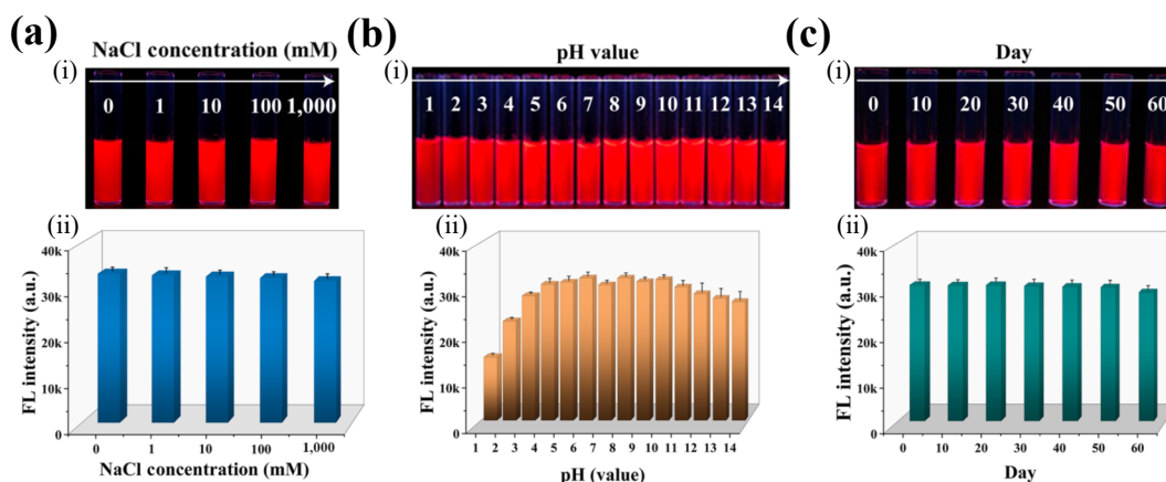
Figure 2 (a)(i) Photograph of GO@TQD nanofilms at various salt concentrations under 365 nm UV light and (ii) their corresponding fluorescence intensities at the maximum emission wavelength. (b)(i) Photographs and (ii) detailed fluorescence signals of GO@TQD nanosheets at various pH levels. (c)(i) Photographs and (ii) detailed fluorescence signals of GO@TQD nanofilms dispersed in ethanol against preservation time.
