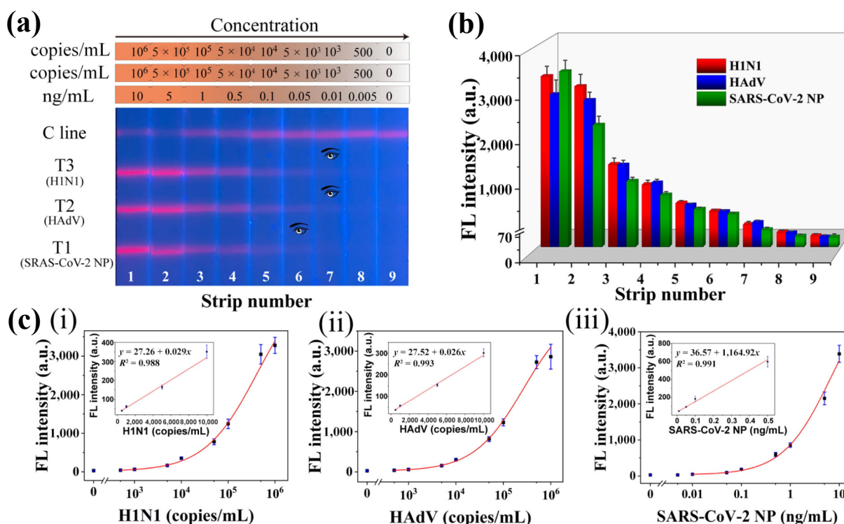
Figure 4 (a) Fluorescence images and (b) corresponding signal intensities on test lines of GO@TQD-LFA strips for detection of SARS-CoV-2 NP, HAdV, and H1N1. (c) Corresponding calibration curves for (i) H1N1, (ii) HAdV, and (iii) SARS-CoV-2 NP.
