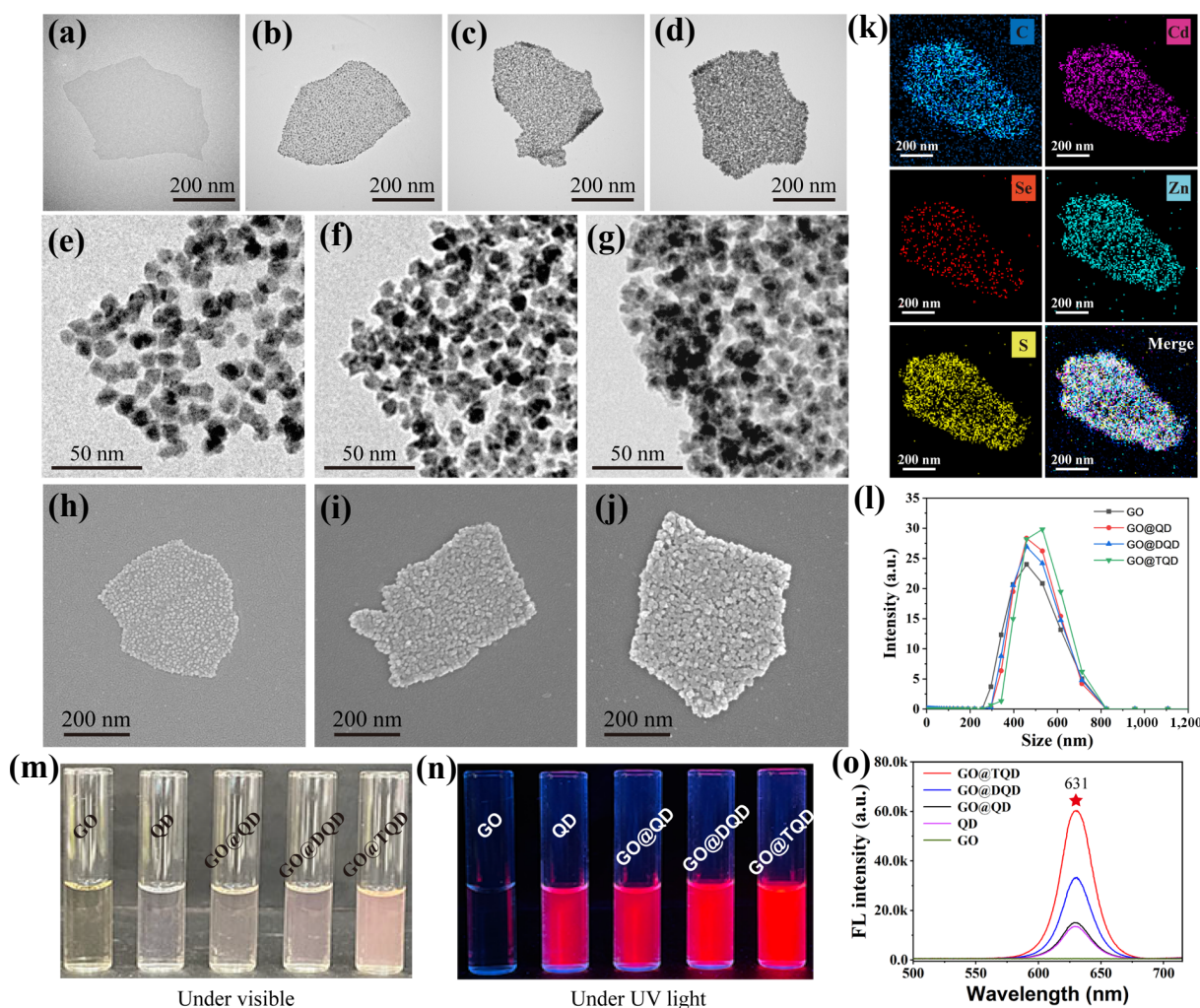
Figure 1 Structural characterization of the prepared GO@TQD nanofilm. TEM images of (a) GO, (b) GO@QD, (c) GO@DQD, and (d) GO@TQD nanofilms. Enlarged TEM images of (e) GO@QD, (f) GO@DQD, and (g) GO@TQD nanofilms. SEM images of (h) GO@QD, (i) GO@DQD, and (j) GO@TQD nanofilms. (k) EDS elemental maps of C, Cd, Se, Zn, and S signals on a single GO@TQD nanofilm. (l) Dynamic light scattering distribution of GO, GO@QD, GO@DQD, and GO@TQD. The x- and y- coordinate represent the size (nm) of the nanofilms and the relative signal intensity, respectively. (m) and (n) Photographs and (o) fluorescence emission spectra of GO, QD, GO@QD, GO@DQD, and GO@TQD nanofilms.
